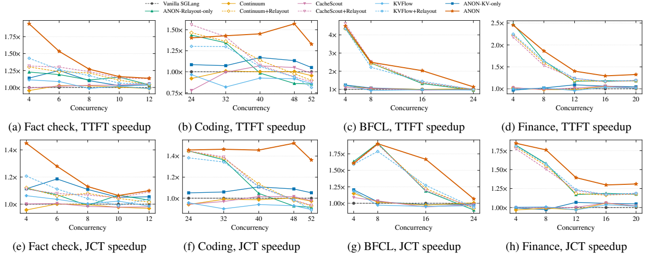
Figure 5. Average TTFT speedup (top) and average JCT speedup (bottom) over Vanilla SGLang under varying numbers of concurrent workflows.
