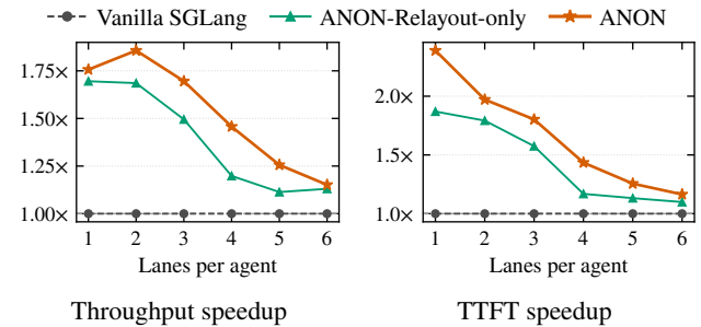
Figure 4. Throughput and average TTFT speedup over Vanilla SGLang on different pressure of mixed workloads.
