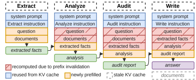
Figure 1. Recompute and KV-cache status demonstration in a four-stages financial-analysis agent. It answers the question using the given documents. The the stage-specific task instructions block KV-cache reuse, and serving engine cannot proactively release the stale KV cache ( documents after Audit here) without knowing the intra-prompt heterogeneity.
