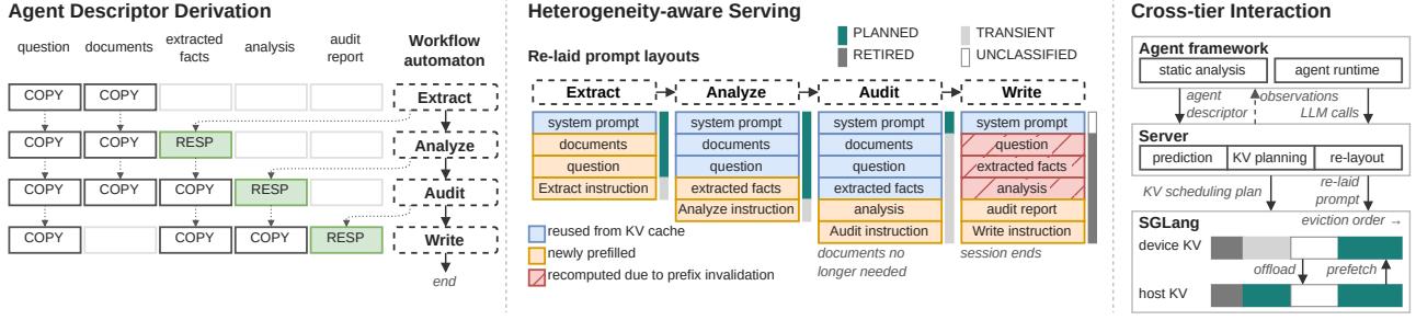
Figure 3. Architecture overview of ANON. Static Analysis derives agent descriptor, mark the intra-prompt heterogeneity. Server side then utilizes it for ANON’s efficient KV-cache scheduling.
