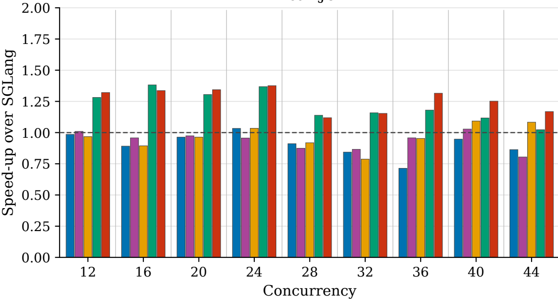
Mean JCT
