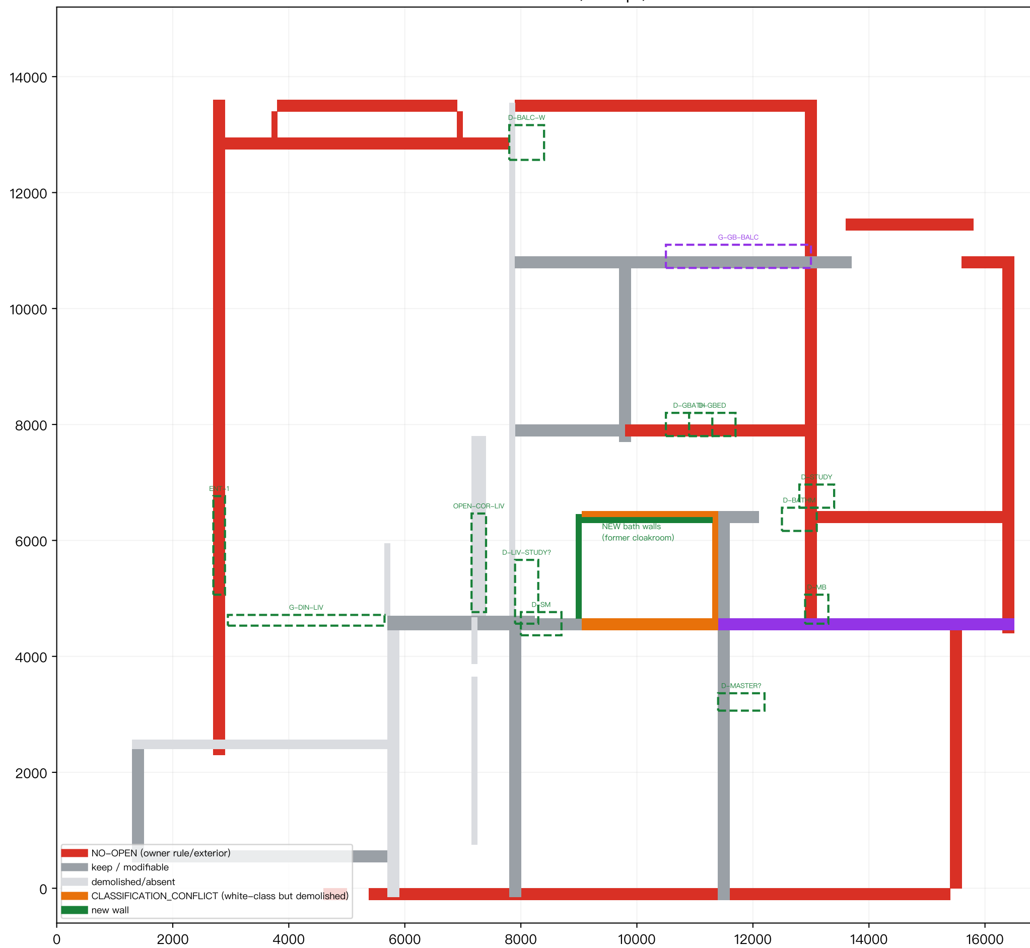
Task03A · Demolition / Keep / New
