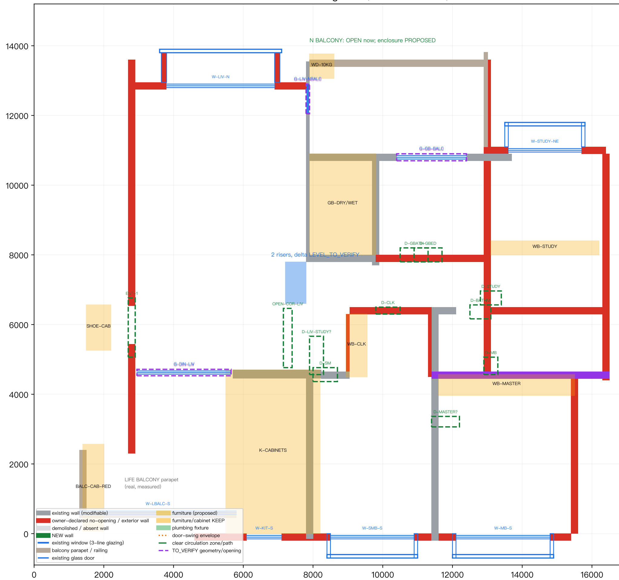
Task03A · Current Existing Plan (measured DWG)
