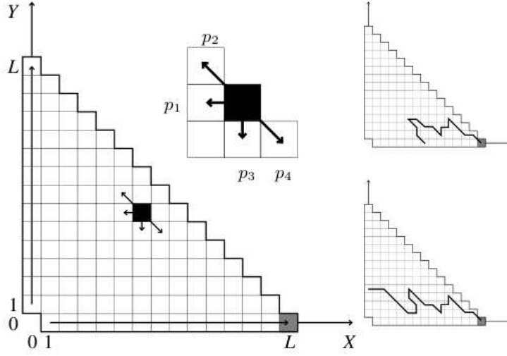
Figure 1.44: Phase space of the bridge model for \beta \ll 1 and schematic of dynamics. The gray site of coordinates (L, 0) is the initial configuration (bridge filled with negative particles) and the black site is a generic configuration whose allowed transitions are indicated by the four arrows. Each move has a probability p_i , given in Eq. (4.46). On the right we sketch
