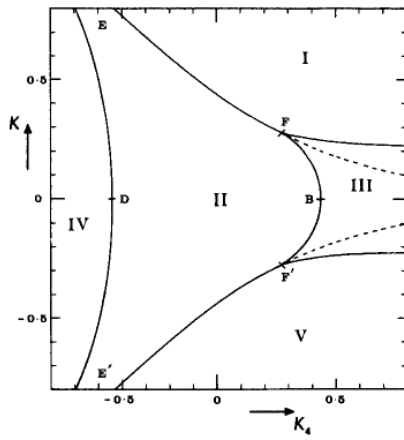
Fig. 12.12. Phase diagram of the isotropic Ashkin – Teller model, in (K_4, K)
