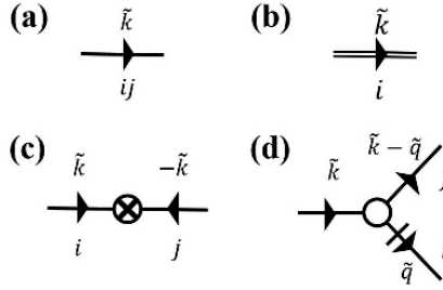
Fig. 9.4.1 Rules of graphical representation: (a) G_{ij}(\tilde{\mathbf{k}}) ; (b) u_i^\perp(\tilde{\mathbf{k}}) ; (c) 2DC_{ij}(\tilde{\mathbf{k}}) ; (d) the nonlinear term proportional to -\mathrm{i}\lambda_1 ; the slash represents a factor q_j^\perp . Reproduced from [23].
