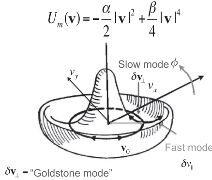
Fig. 4.2.3 The “Mexican hat” potential. Note the circular ring of minima. Fluctuations \delta \mathbf{v}_\perp of the velocity that move it around this ring are “Goldstone modes,” which experience no restoring force from this “potential.” In contrast, fluctuations \delta v_\parallel that carry one up the brim of the hat, or towards the crown (i.e., radially), are “fast”; i.e., they will relax quickly due to this potential, which simply reflects the existence of a preferred speed for the flocks’ motion through the frictional medium. Reproduced from [7] by permission of Oxford University Press.
