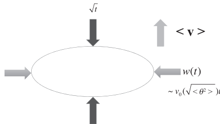
Fig. 7.2.1 Correct picture of the evolving blob. It still grows diffusively in the direction of the mean flock velocity (vertical in this figure), but grows laterally at a rate dominated by motion of the flockers (i.e., convection), rather than diffusion. This convective width w(t) can be determined self-consistently via equation (7.2.5). Reproduced from [7] by permission of Oxford University Press.
