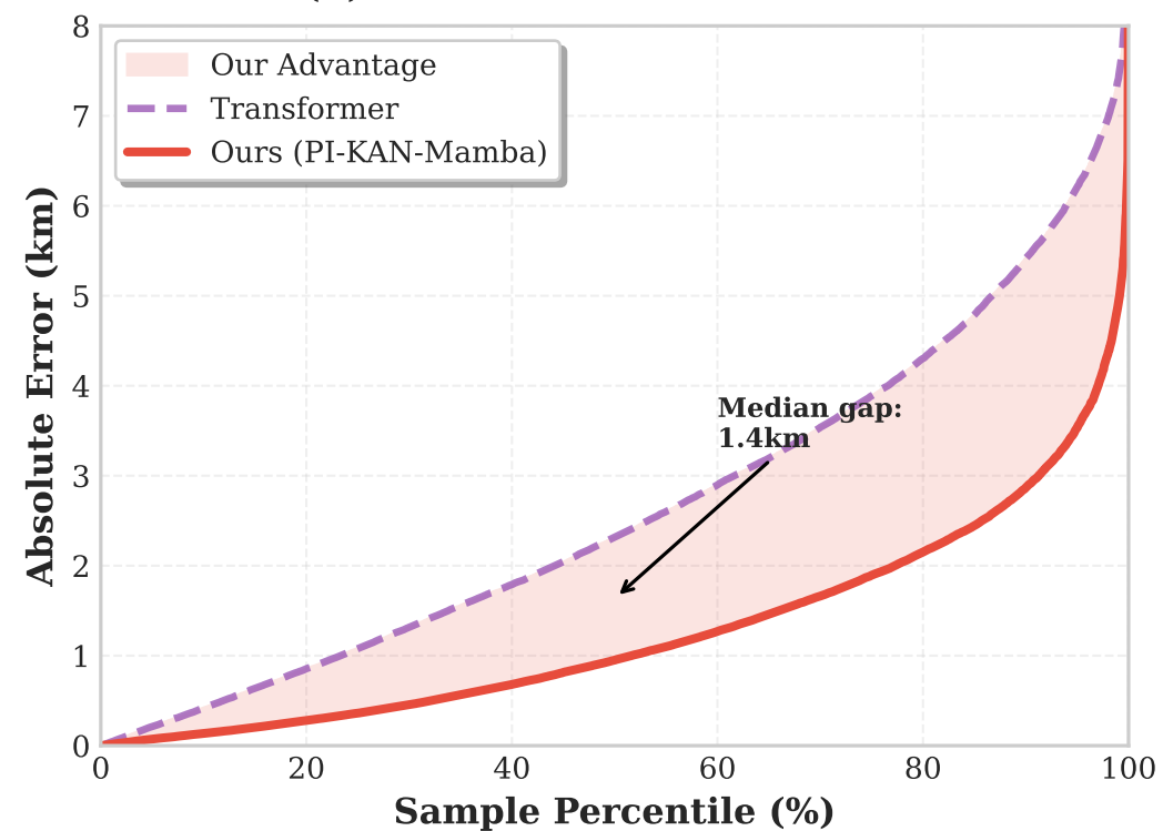
(b) Sorted Error Distribution
