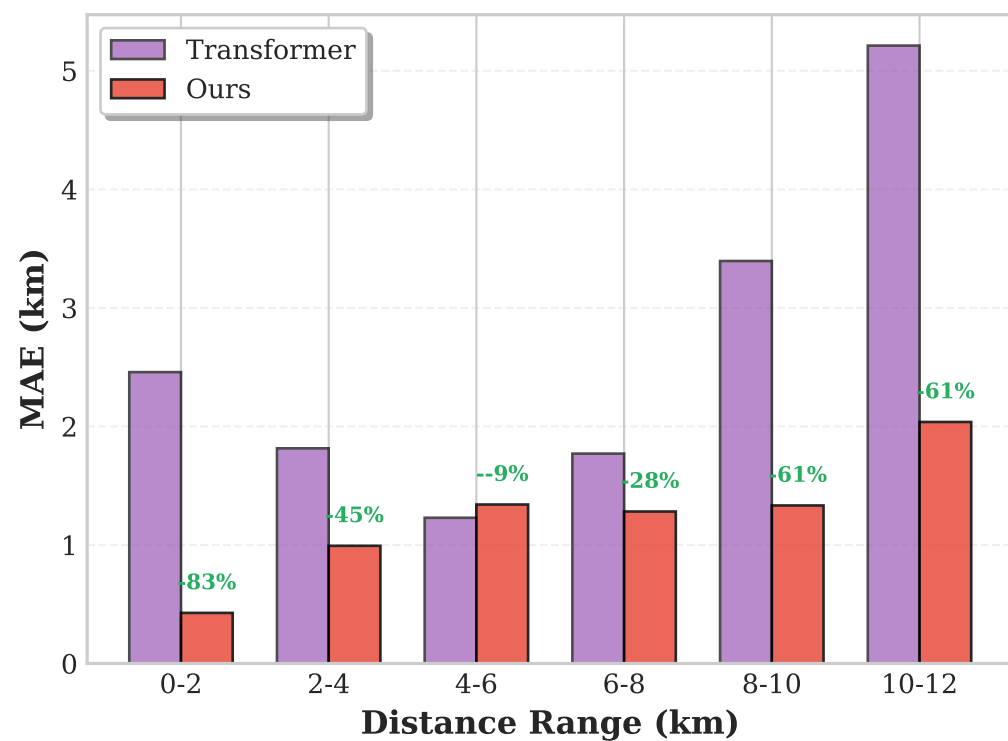
(c) MAE by Distance Range
