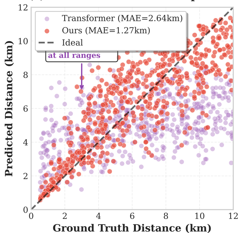
(a) Prediction Scatter Comparison
