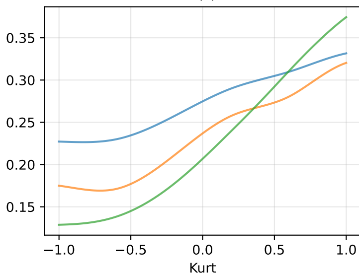
Learned f(x) for Kurt
