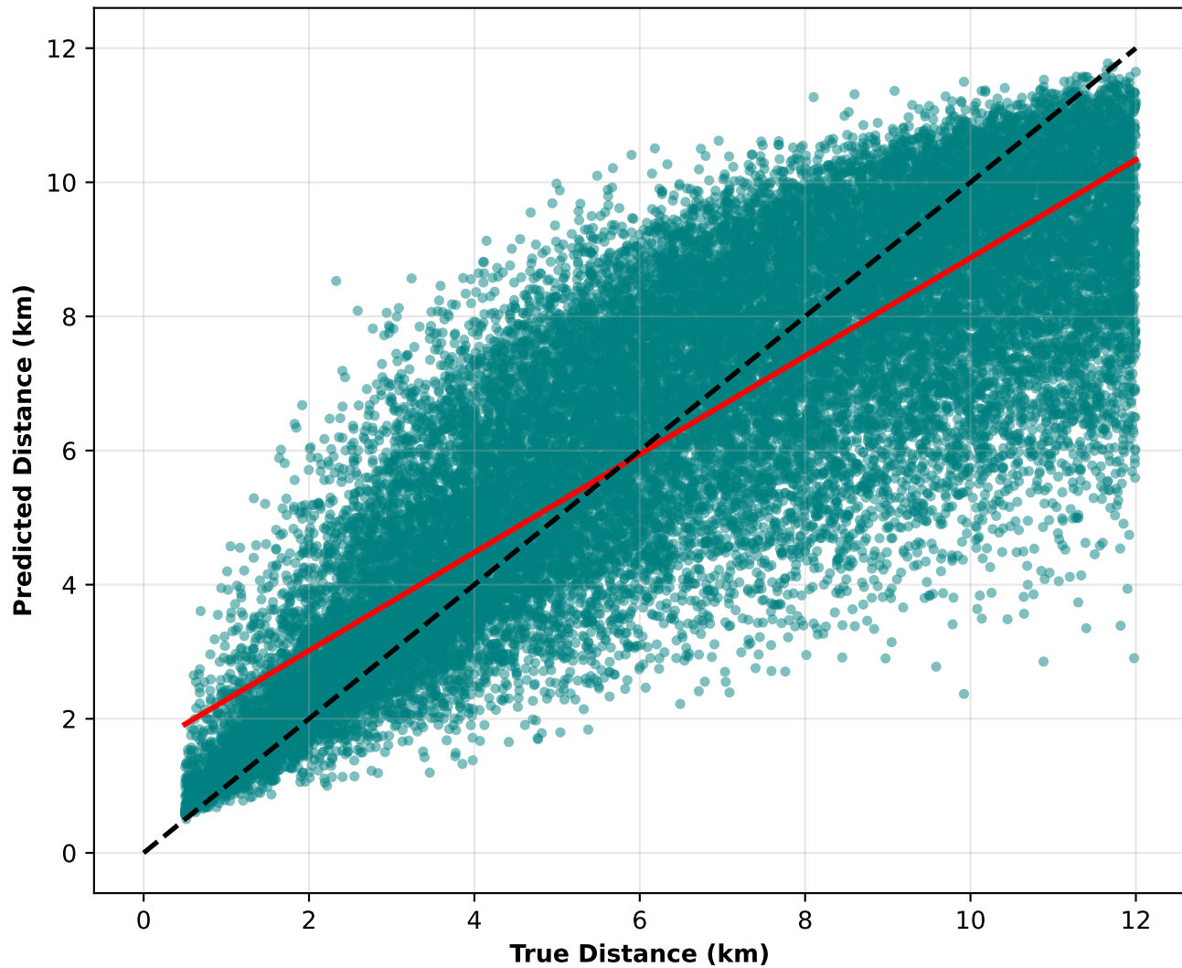
Prediction Scatter (MAE=1.276km, R 2 =0.729)
