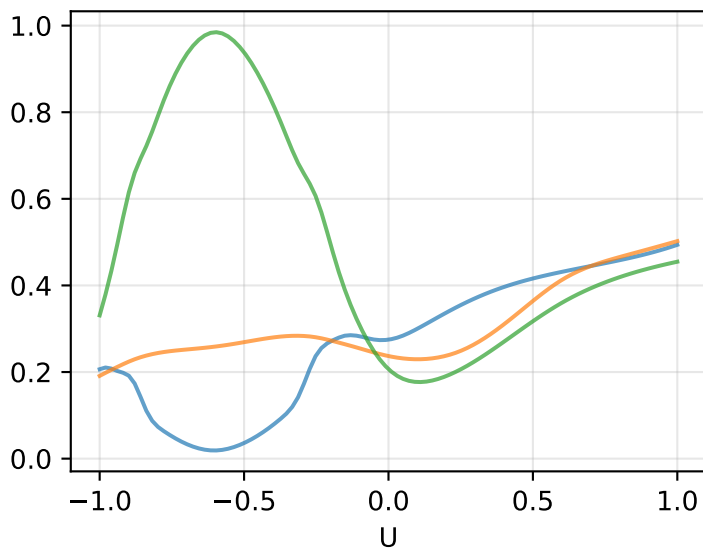
Learned f(x) for Kurt
