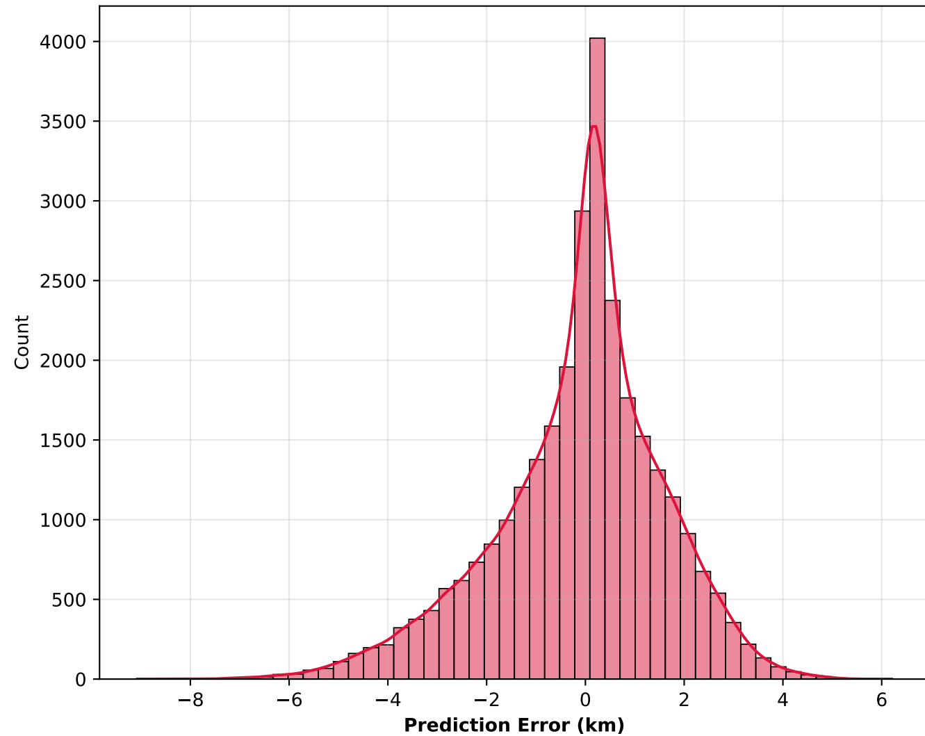
Error Distribution
