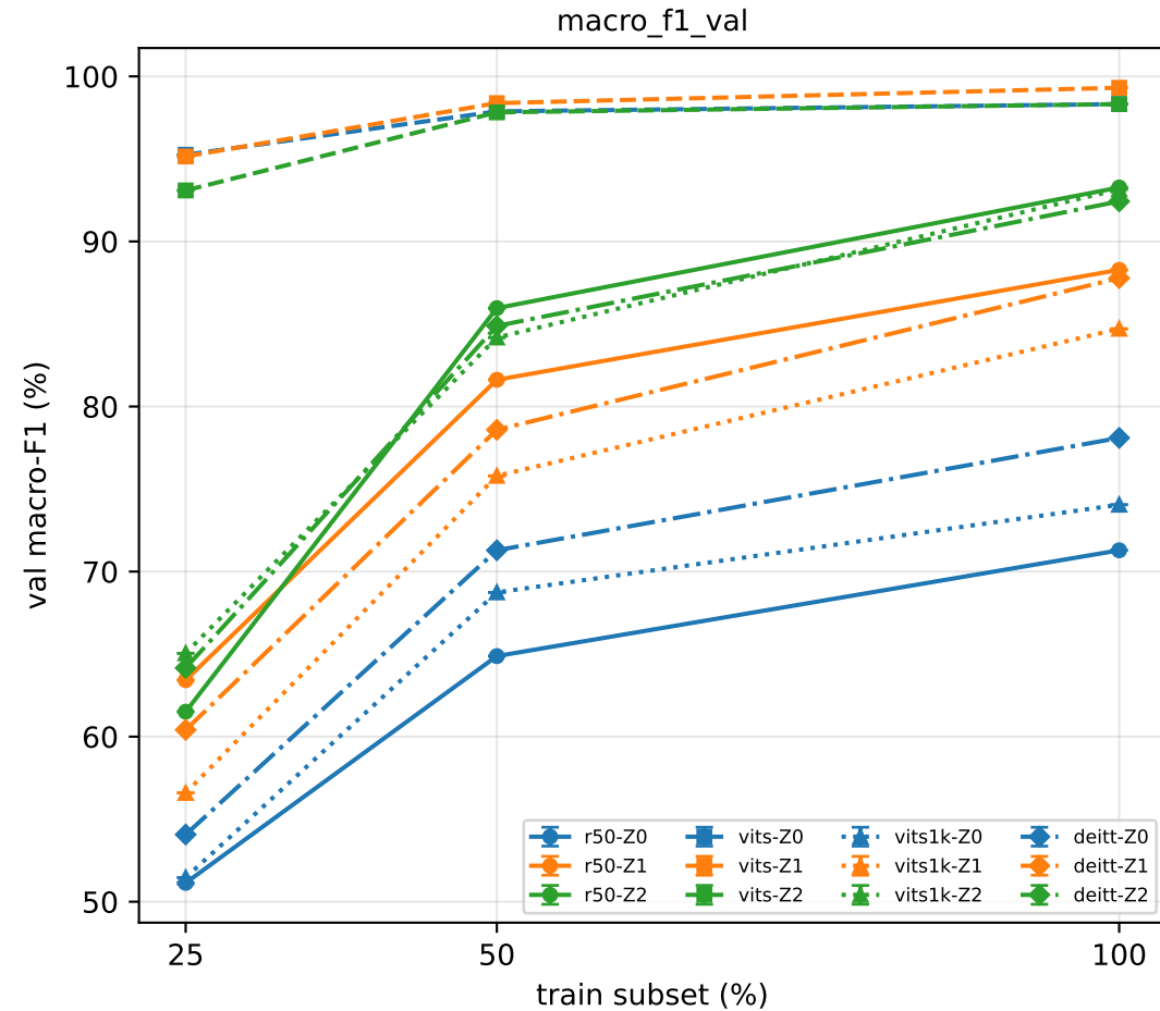
W5 C1 ladder - color = strategy (Z0/Z1/Z2), line+marker = arch (vits1k = dotted/^)
