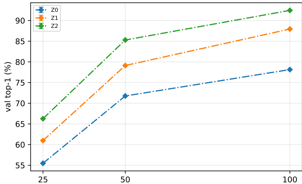
deitt
