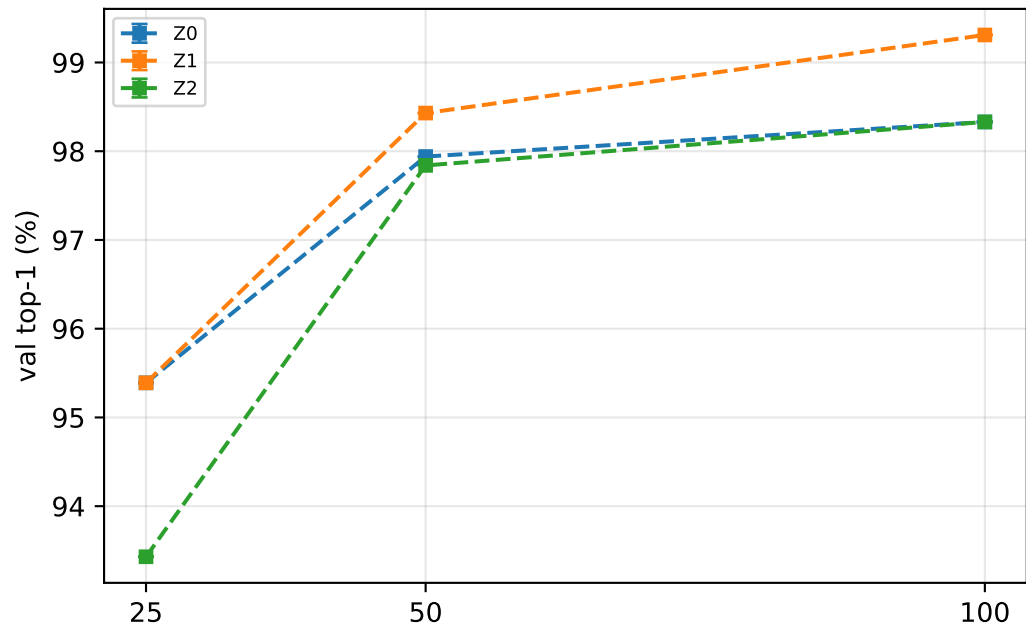
deitt
