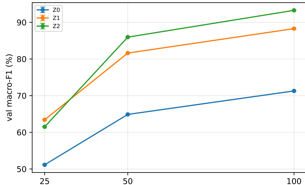
W5 C1 ladder - macro_f1_val (one panel per arch; color = strategy)
