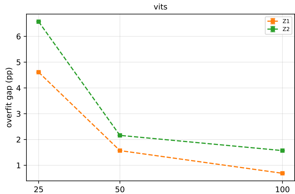
W5 C1 ladder - gap (one panel per arch; color = strategy)
