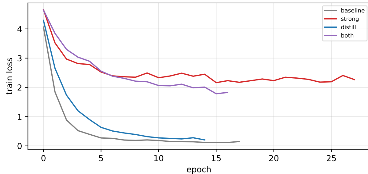
25% - train loss
