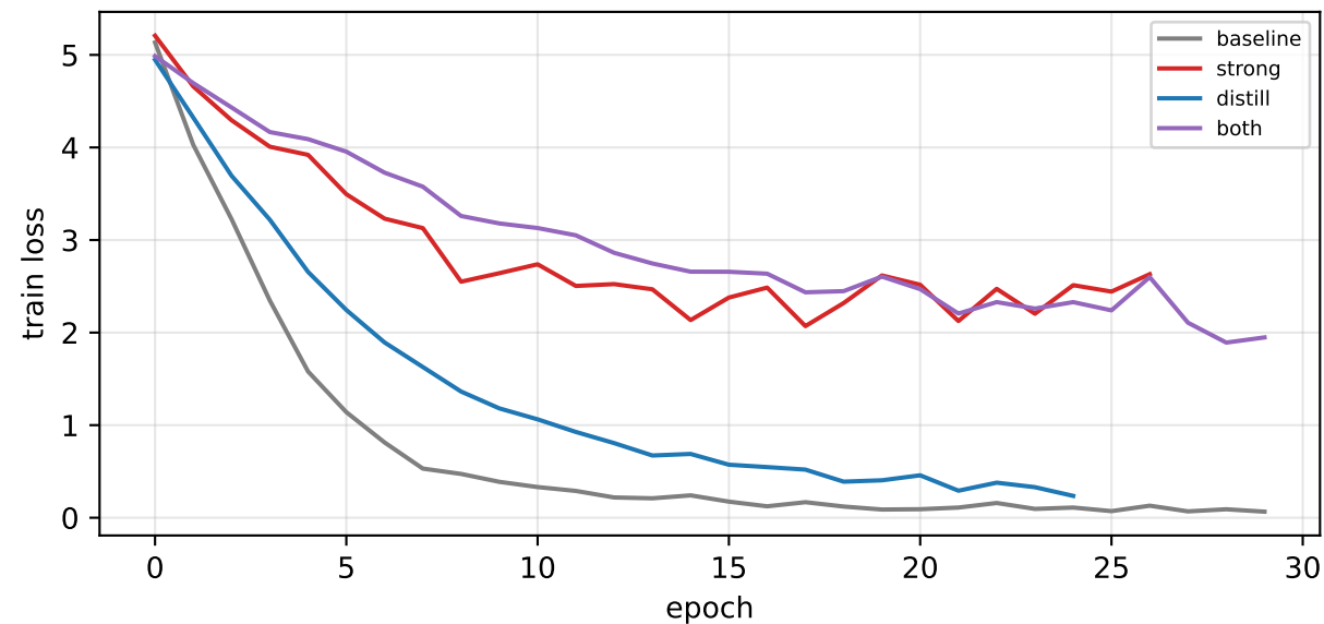
25% - train loss
