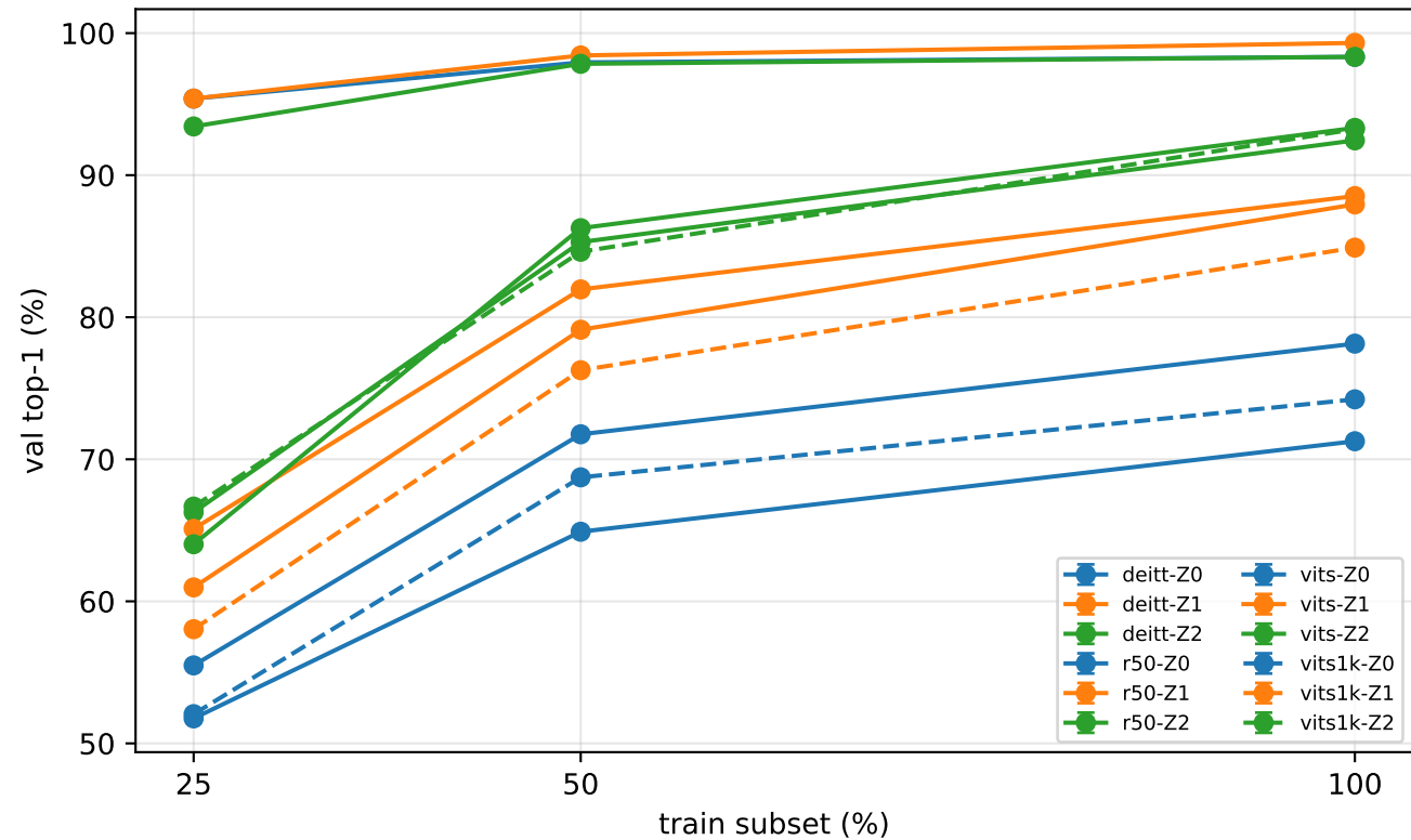
W5 C1 ladder - top1_val
