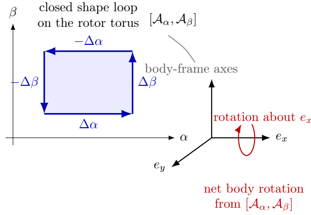
Figure 8.3: Helicopter-rotor gauge laboratory. The connection components are constant, but they point in noncommuting body directions. A closed rectangle in shape space therefore has curvature from the commutator term and can produce a net body rotation.
