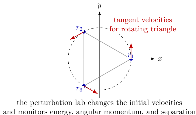
Figure 6.3: Equal-mass three-body laboratory. The unperturbed comparison solution starts from an equilateral triangle with tangential velocities; perturbing this initial data is a controlled way to watch the loss of symmetric motion.
