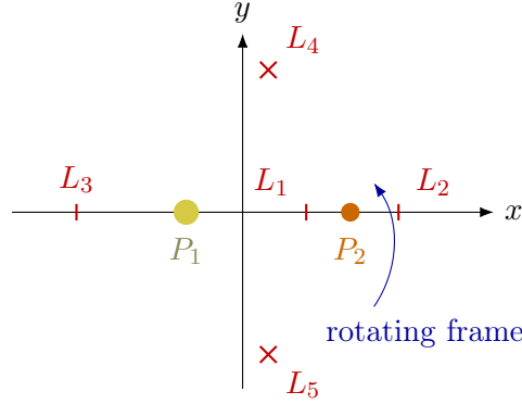
Figure 6.1: Circular restricted three-body geometry in rotating barycentric coordinates. The primaries are fixed, while the test particle moves under gravity, centrifugal force, and Coriolis deflection.
