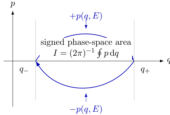
Figure 4.5: For a one-dimensional bound orbit the action is the signed phase-space area enclosed by the energy curve divided by 2\pi . The turning points contribute no endpoint term when differentiating with respect to energy because p(q_{\pm}, E) = 0 .
