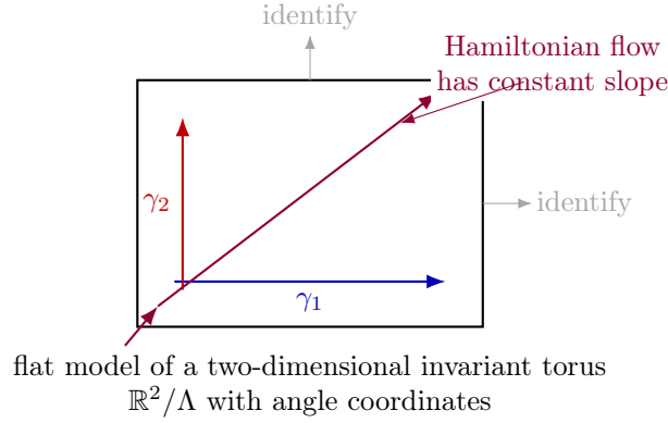
Figure 4.4: A Liouville torus is locally a space of commuting flow times with periodic identifications. Action variables label the torus; angle variables are coordinates along the fundamental cycles.
