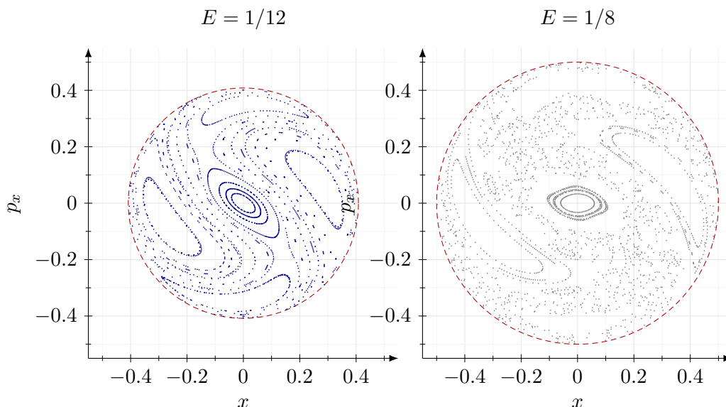
Figure 5.5: Numerical Poincare sections of the Henon-Heiles flow on y = 0 , p_y > 0 . Each plotted point is an upward section crossing from a velocity-Verlet integration of the Hamiltonian in the text. The dashed red circle is the kinematic boundary x^2 + p_x^2 = 2E on the section, where p_y = 0 . At E = 1/12 the section is dominated by deformed invariant curves; by E = 1/8 a chaotic sea coexists with surviving islands and smaller regular regions.
