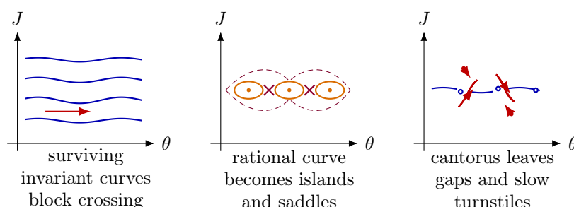
Figure 5.3: Three stages in the loss of transport barriers on a two-dimensional section. Left: invariant curves separate the annulus. Middle: a rational curve splits into an island chain with hyperbolic points. Right: an irrational curve may leave a cantorus, which permits transport only through gaps.
