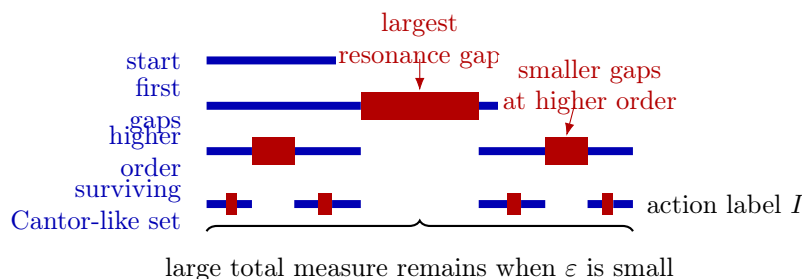
Figure 5.2: KAM survival is Cantor-like. Resonant action labels are removed in thin layers around k \cdot \omega = 0 ; the surviving Diophantine labels are nowhere all of the line, but their total measure approaches the integrable measure as \varepsilon \rightarrow 0 .
