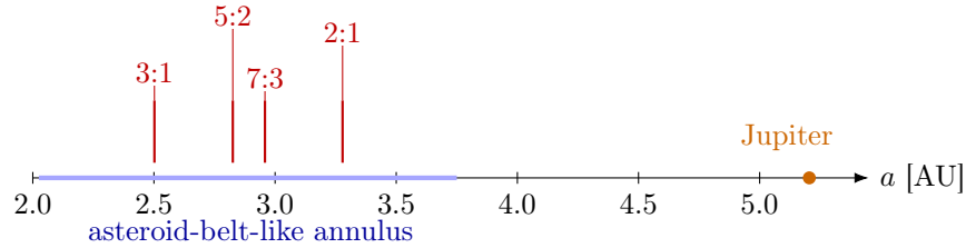
Figure 5.1: Nominal mean-motion resonance locations with Jupiter, shown across an asteroid-belt-like range. The resonance positions use a_{p:q} = a_J(q/p)^{2/3} ; the figure now includes Jupiter's orbital radius to show that the listed resonances lie interior to Jupiter.
