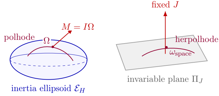
Figure 4.3: Poincaré construction. In body angular-velocity space, the motion lies on the inertia ellipsoid and traces the polhode. In space, the tip of angular velocity lies in the fixed invariant plane perpendicular to the conserved spatial angular momentum J ; its trace is the herpolhode.
