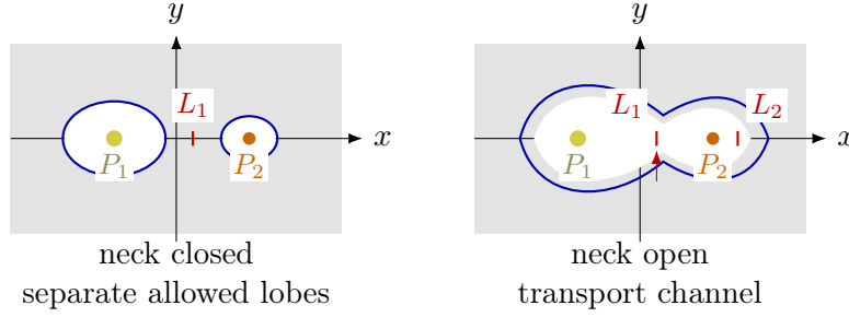
Figure 6.2: Schematic zero-velocity curves in the rotating CR3BP plane. Gray regions are forbidden by 2\Omega_{\text{eff}} < C_J ; white regions are allowed projections of the energy surface. Changing C_J can open a neck near L_1 , creating a channel between previously separated regions.
