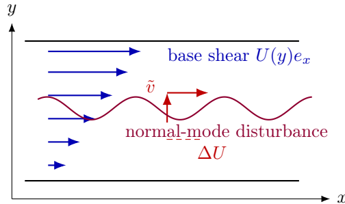
Figure 9.4: Linear shear-flow stability. A wall-normal perturbation velocity \tilde{v} moves fluid across the base shear; the term \tilde{v} U'(y) e_x is the linear energy-exchange channel between the base flow and the disturbance.
