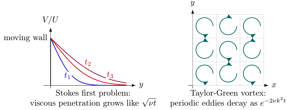
Figure 9.3: Two unsteady exact solutions, drawn by evaluating the formulas in the text rather than by numerically integrating Navier-Stokes. Left: an impulsively moved wall creates the profile V/U = \text{erfc}(y/(2\sqrt{\nu t})) . The horizontal axis is the distance y from the wall, the vertical axis is the normalized velocity V/U , and the three curves show increasing times t_1 < t_2 < t_3 ; the growing penetration depth is the viscous scale \sqrt{\nu t} . Right: the square is one periodic x, y cell of the Taylor-Green velocity (A \sin kx \cos ky, -A \cos kx \sin ky) . The curved arrows indicate the alternating eddy circulation; advection is absorbed by pressure while viscosity damps the common amplitude by e^{-2\nu k^2 t} .
