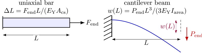
Figure 7.3: Two classical reductions of three-dimensional linear elasticity. A slender bar under axial load measures Young's modulus. A slender beam under transverse load converts elastic energy in curvature into the fourth-order Euler-Bernoulli equation.
