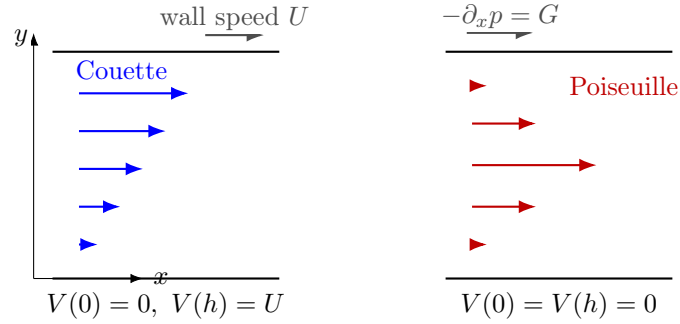
Figure 9.2: Two steady shear profiles between parallel plates separated by distance h . In both panels the vertical direction in the drawing is the wall-normal coordinate y , with y = 0 at the lower wall and y = h at the upper wall; the horizontal arrow length represents the streamwise velocity component V(y) . Left: Couette flow, V(0) = 0 and V(h) = U , is linear because it is driven by wall motion. Right: Poiseuille flow, V(0) = V(h) = 0 , is parabolic because it balances the pressure force -\partial_x p = G against viscous diffusion of momentum. The arrows are spatial velocity vectors, not a graph with velocity on the vertical axis.
