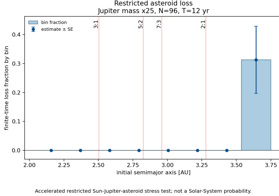
Figure 6.6: Accelerated restricted asteroid-loss benchmark generated by demos/python/three_body_benchmark_studies.py . The horizontal axis is the initial asteroid semimajor axis a_0 in astronomical units, binned into the displayed intervals. The vertical axis is the finite-time loss fraction in each bin after the stated integration horizon. A loss means ejection, collision with the Sun, or close approach to Jupiter according to the absorbing rules in the script. Each blue rectangle is one semimajor-axis bin: its width is the bin interval in a_0 , and its height is the measured fraction N_{\text{loss}}/N_{\text{bin}} . The blue dots mark the same bin estimates with plug-in binomial standard-error bars; dots on the baseline are bins with N_{\text{loss}} = 0 , for which the rectangle has zero height and the error whisker has zero length. Thus a dot sitting on the horizontal axis is not an extra data set; it is the bin-center marker for a zero-loss bin. In the quick run shown here, the only nonzero bin is the last interval, 3.5375 \text{ AU} \leq a_0 \leq 3.75 \text{ AU} , where 5 of 16 sampled particles are lost, giving N_{\text{loss}}/N_{\text{bin}} = 5/16 = 0.3125 . The red vertical lines mark nominal low-order Jovian resonances. Jupiter’s mass is deliberately scaled up to make a short classroom run visibly lossy; the figure is a stress test of the resonance-loss pipeline, not an estimate of the real asteroid-belt loss probability.
