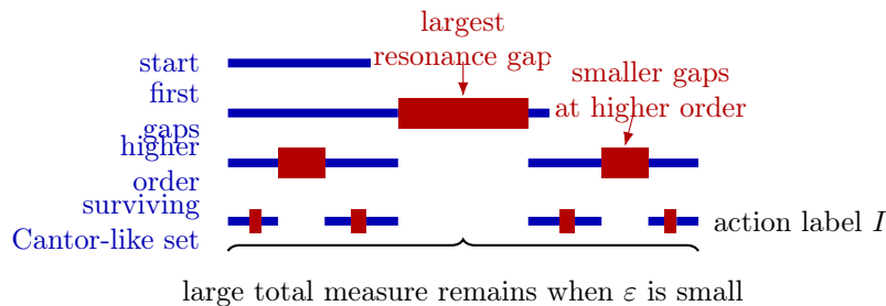
Figure 5.4: KAM survival is Cantor-like. Resonant action labels are removed in thin layers around k \cdot \omega = 0 ; the surviving Diophantine labels are not a continuous interval, but their total measure approaches the integrable measure as \varepsilon \rightarrow 0 when the Diophantine threshold is allowed to shrink with the perturbation size.
