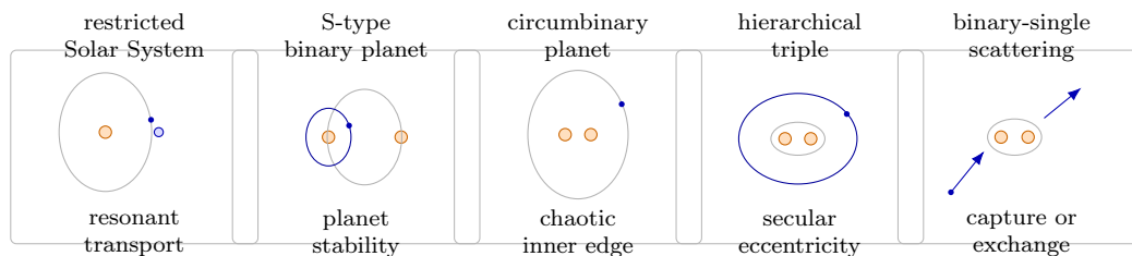
Figure 6.1: Five astrophysical regimes of the three-body problem. The diagrams look different, but the mechanical questions are the same: choose a reference Kepler problem when one exists, identify the slow perturbations, and define a finite-time stability, escape, capture, or exchange observable.
