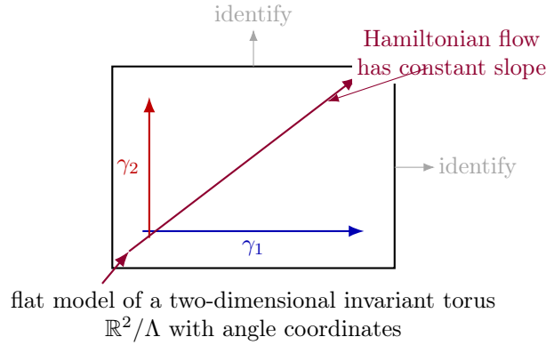
Figure 4.6: A Liouville torus is locally a space of commuting flow times with periodic identifications. Action variables label the torus; angle variables are coordinates along the fundamental cycles.
