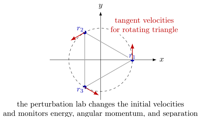
Figure 6.8: Equal-mass three-body laboratory. The unperturbed comparison solution starts from an equilateral triangle with tangential velocities; perturbing this initial data is a controlled way to watch the loss of symmetric motion.
