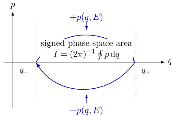
Figure 4.7: For a one-dimensional bound orbit the action is the signed phase-space area enclosed by the energy curve divided by 2\pi . The turning points contribute no endpoint term when differentiating with respect to energy because p(q_{\pm}, E) = 0 .
