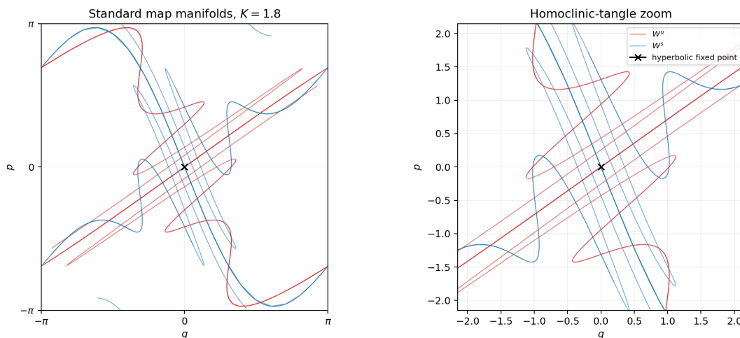
Figure 5.5: Stable and unstable manifolds for the hyperbolic fixed point (q, p) = (0, 0) of the standard map, generated by demos/python/standard_map_homoclinic_tangle.py . Both panels use the centered torus coordinates (q, p) \in [-\pi, \pi) \times [-\pi, \pi) , and the map is p_{n+1} = p_n + K \sin q_n , q_{n+1} = q_n + p_{n+1} modulo 2\pi , with K = 1.8 chosen so the splitting and folds are visible at lecture-note scale. The black cross is the hyperbolic fixed point. The red curves approximate W^u , the unstable manifold, by forward iterates of a tiny segment tangent to the unstable eigenvector of the linearized map. The blue curves approximate W^s , the stable manifold, by inverse iterates of a tiny segment tangent to the stable eigenvector. The left panel shows the computed manifold branches on the torus; the right panel restricts the view to a smaller square so the transverse red-blue crossings and folds of the homoclinic tangle are easier to see. These are finite numerical images of local tangent segments, not a complete global parametrization of W^s \cup W^u .
