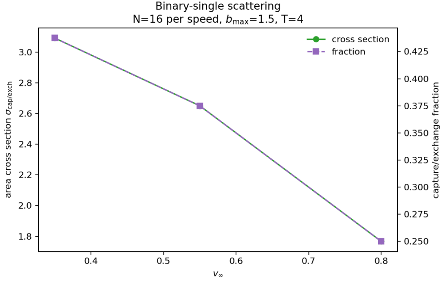
Finite-horizon binary-single classifier; capture/exchange is ensemble and stopping-rule dependent.
