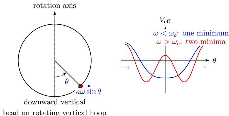
Figure 2.4: Rotating-hoop laboratory. The geometry fixes the kinetic term a^2\omega^2 \sin^2 \theta , and the effective potential changes from one bottom minimum to two off-bottom minima when \omega crosses \omega_c = \sqrt{g/a} . The potential curves are schematic and emphasize the bifurcation, not numerical scale.
