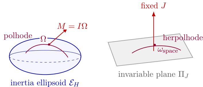
Figure 4.3: Poincaré construction. In body angular-velocity space, the motion lies on the inertia ellipsoid and traces the polhode. In space, the tip of angular velocity lies in the fixed invariable plane perpendicular to the conserved spatial angular momentum J ; its trace is the herpolhode.
