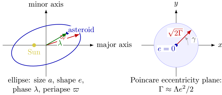
Figure 5.1: Planar Poincare variables replace the singular periaipse angle at e = 0 by Cartesian eccentricity coordinates. The action \Lambda measures semimajor axis, while \Gamma measures eccentricity to leading order.
