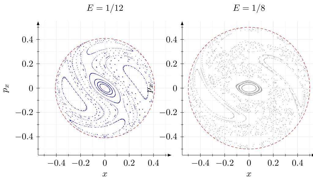
Figure 5.8: Numerical Poincaré sections of the Henon-Heiles flow on y = 0 , p_y > 0 , generated from the data files written by demos/python/henon_heiles_poincare.py . In each panel the horizontal axis is x and the vertical axis is p_x , both in the nondimensional units of the Hamiltonian in the text. The integration records one point each time the orbit crosses the section upward; p_y is then determined by the fixed energy and is not an independent plotted coordinate. The dashed red circle is the kinematic boundary x^2 + p_x^2 = 2E on the section, where p_y = 0 . At E = 1/12 the section is dominated by deformed invariant curves; by E = 1/8 a chaotic sea coexists with surviving islands and smaller regular regions.
