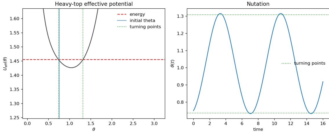
Figure 4.5: Numerical heavy-top laboratory generated by demos/python/heavy_symmetric_top.py . The left panel has horizontal axis \theta , the polar angle between the body symmetry axis and the vertical, and vertical axis U_{\text{eff}}(\theta) in the nondimensional units of the script. The conserved momenta p_\phi and p_\psi are held fixed; the dashed horizontal line is the conserved reduced energy, and the vertical marker is the initial value of \theta . Intersections of the energy line with U_{\text{eff}} are the nutation turning points; the green dotted vertical lines mark those angles. The right panel uses the same reduced model: its horizontal axis is nondimensional time and its vertical axis is the numerically integrated angle \theta(t) . The green dotted horizontal lines are the same turning-point angles, now drawn as reference levels for \theta(t) . Thus the two panels are not independent experiments; they are the potential picture and the corresponding time trace for one reduced heavy-top problem.
