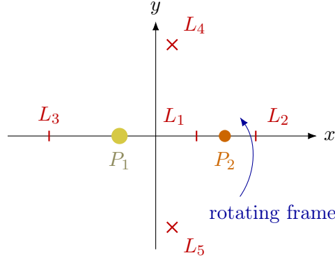
Figure 6.4: Circular restricted three-body geometry in rotating barycentric coordinates. The primaries are fixed, while the test particle moves under gravity, centrifugal force, and Coriolis deflection.
