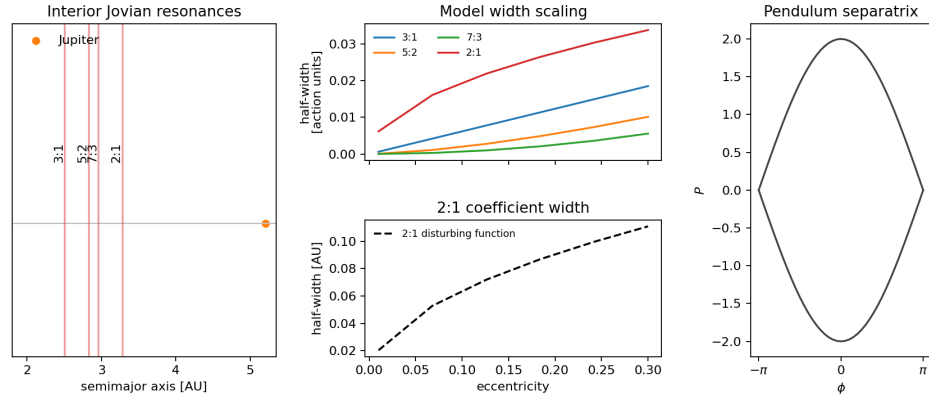
Figure 5.3: Numerical companion to the resonant normal-form calculation, generated by demos/python/asteroid_resonance_normal_form.py . The left panel uses semimajor axis a in astronomical units on the horizontal axis; the vertical resonance markers are the nominal interior Jovian resonances a_{p:q} = a_J(q/p)^{2/3} , and the Jupiter marker identifies a_J , not an asteroid data point. The two middle panels both use eccentricity e on the horizontal axis but deliberately use different vertical scales. The upper middle panel shows the illustrative normal-form half-widths in dimensionless action units for the placeholder model B_r(e) = \eta e^r . The lower middle panel shows only the quantitative 2 : 1 half-width in astronomical units, obtained from the disturbing-function coefficient C_{2:1} in the text. Their heights should not be compared across panels: the separation is meant to avoid mixing model action units with AU. The right panel is the universal pendulum normal form: the horizontal axis is the resonant angle \phi \in [-\pi, \pi] , the vertical axis is its conjugate momentum P in normalized units, and the curve is the separatrix. The panels should be read as location, model-scaling, physical-width, and phase-portrait views of the same resonance calculation, not as an asteroid trajectory.
