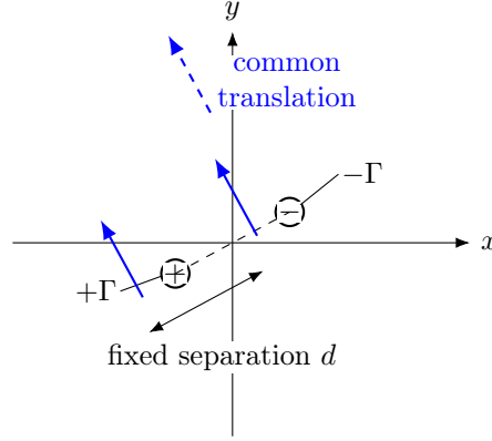
Figure 9.5: Point-vortex dipole in the plane. The displayed axes are spatial coordinates x and y . The two marked singular vortices have equal and opposite circulations +\Gamma and -\Gamma , separated by a fixed distance d . Each blue arrow is the velocity induced at one vortex by the other; because the induced velocities are equal and parallel, the pair translates together without changing separation. More complicated point-vortex systems give finite-dimensional Hamiltonian models of ideal-fluid motion.
