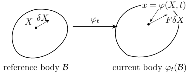
Figure C.1: Material and spatial descriptions are connected by the placement \varphi_t . The deformation gradient F maps material tangent vectors to spatial tangent vectors.
