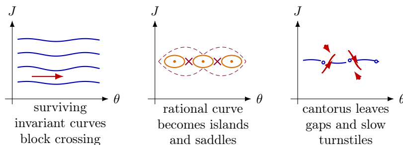
Figure 5.6: Three stages in the loss of transport barriers on a two-dimensional section. Left: invariant curves separate the annulus. Middle: a rational curve splits into an island chain with hyperbolic points. Right: an irrational curve may leave a cantorus, which permits transport only through gaps.
