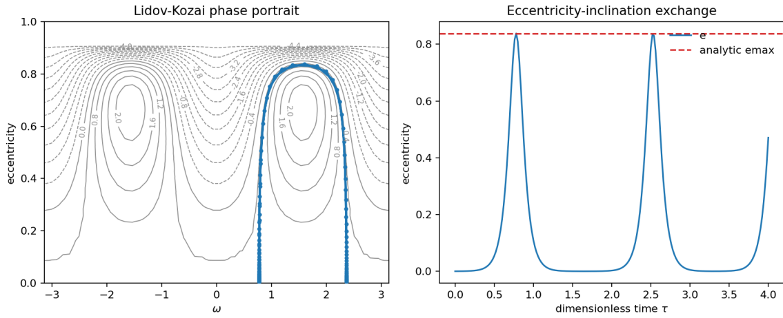
Figure 6.3: Numerical Lidov–Kozai laboratory generated by demos/python/lidov_kozai.py for an orbit initialized near i_0 = 65^\circ with a tiny eccentricity seed. The left panel is the reduced phase portrait at fixed h = \sqrt{1 - e^2} \cos i : the horizontal axis is the argument of periastron \omega and the vertical axis is eccentricity e . Contours are level sets of the quadrupole-averaged Hamiltonian, and the blue curve is one numerically integrated secular trajectory on that same level-set geometry. The inline contour labels are numerical values of the dimensionless Hamiltonian \mathcal{H}_{\text{LK}} used by the script. In the right panel the horizontal axis is the script’s dimensionless secular time \tau , the vertical axis is e(\tau) , the blue curve is the numerical solution, and the dashed red line is the analytic maximum e_{\text{max}} = \sqrt{1 - (5/3) \cos^2 i_0} . The seed is a coordinate regularization because \omega is undefined at exactly e = 0 ; it is not an extra physical perturbation.
