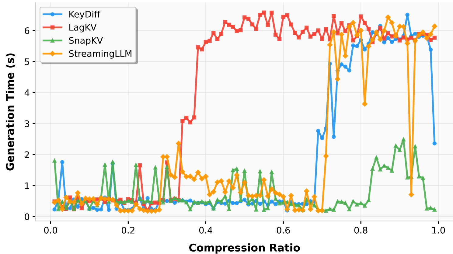
PG19 - Generation Time (s)
