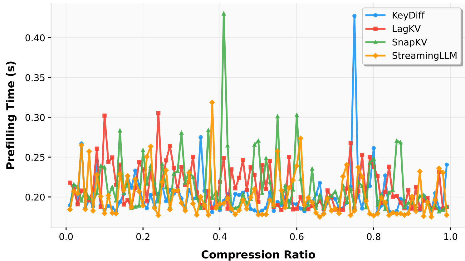
PG19 - Prefilling Time (s)
