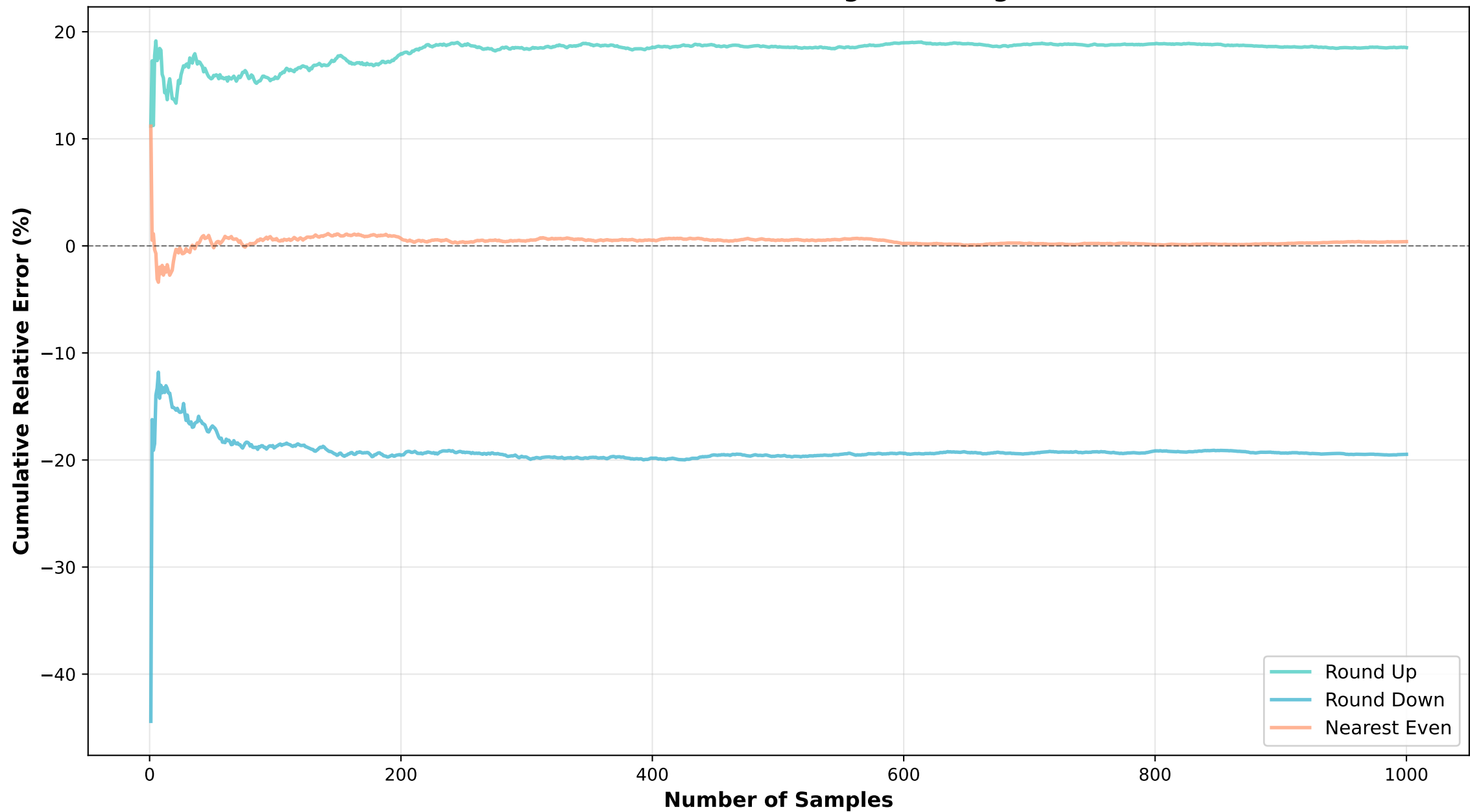
Cumulative Relative Rounding Error Progression
