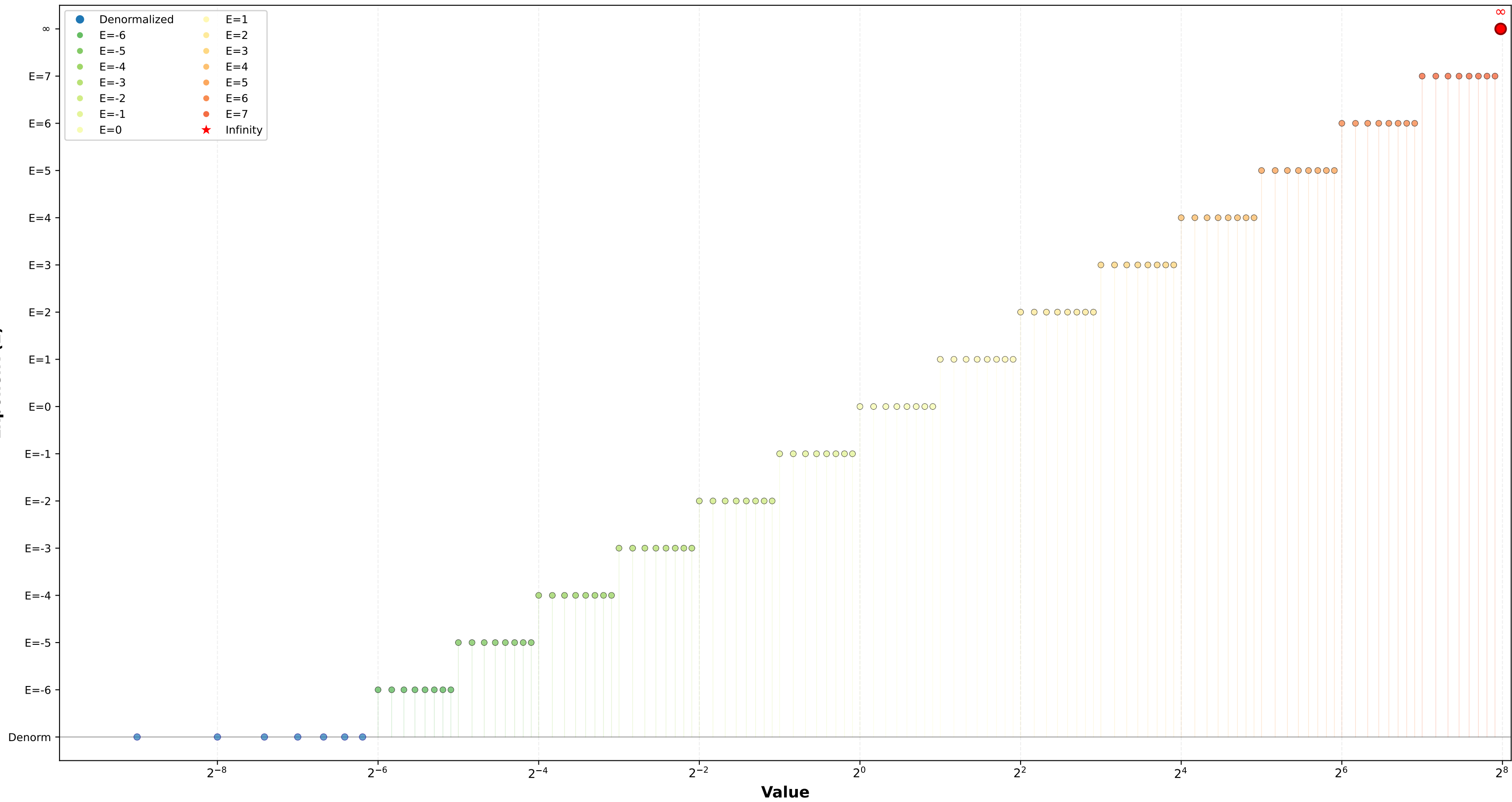
Distribution of Floating-Point Numbers(4-bit exp + 3-bit frac) - Logarithmic Scale
