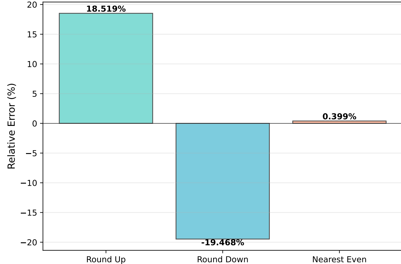
Cumulative Relative Error by Rounding Method
