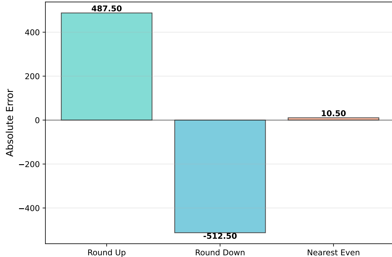
Cumulative Absolute Error by Rounding Method
