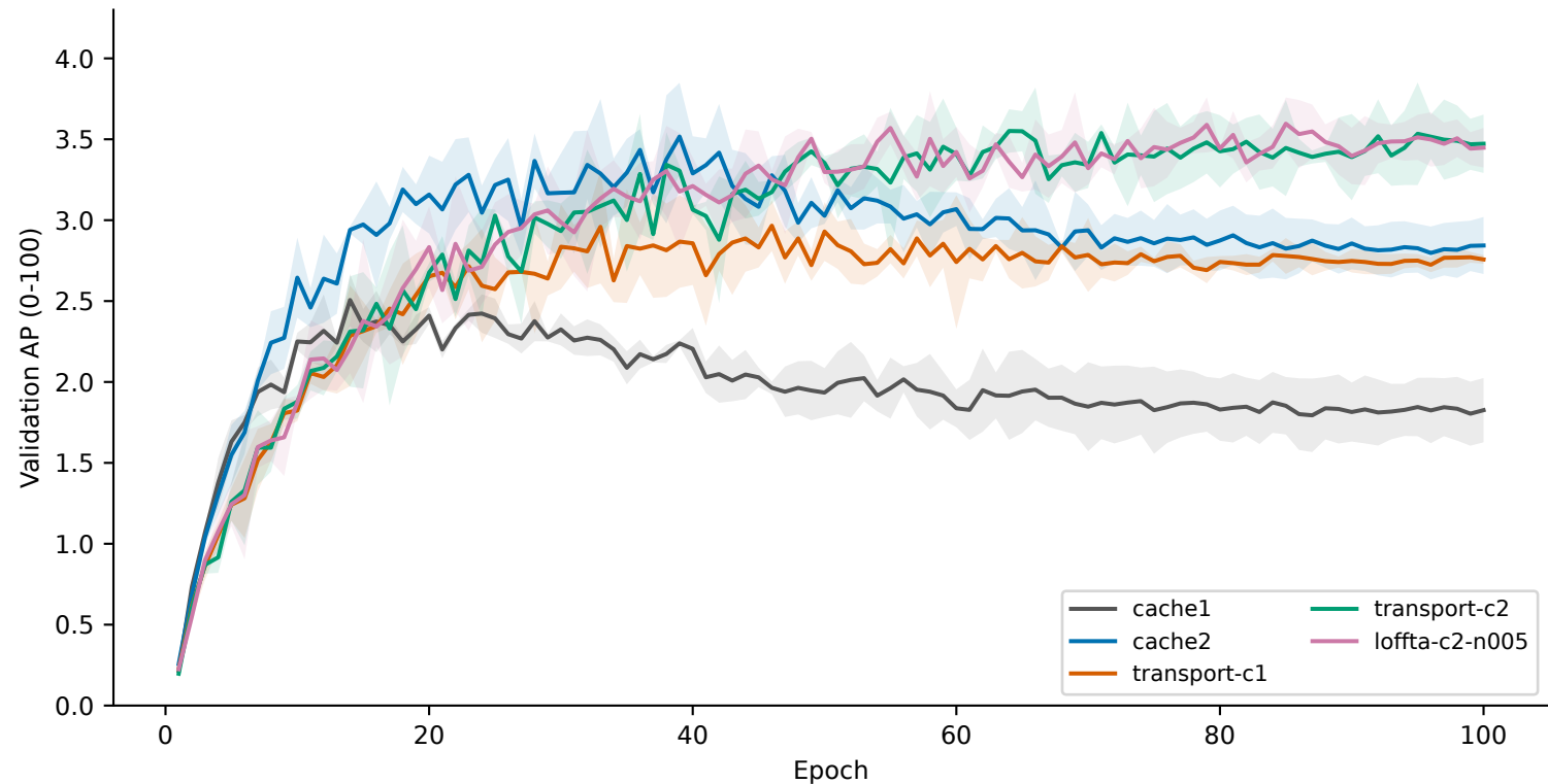
Training dynamics: seed mean and +/- one seed SD
