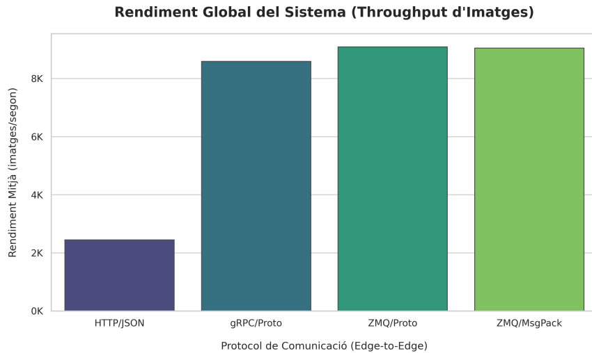
Figura 6.1: Comparativa de rendiment brut ( Throughput ) processant tensors.
