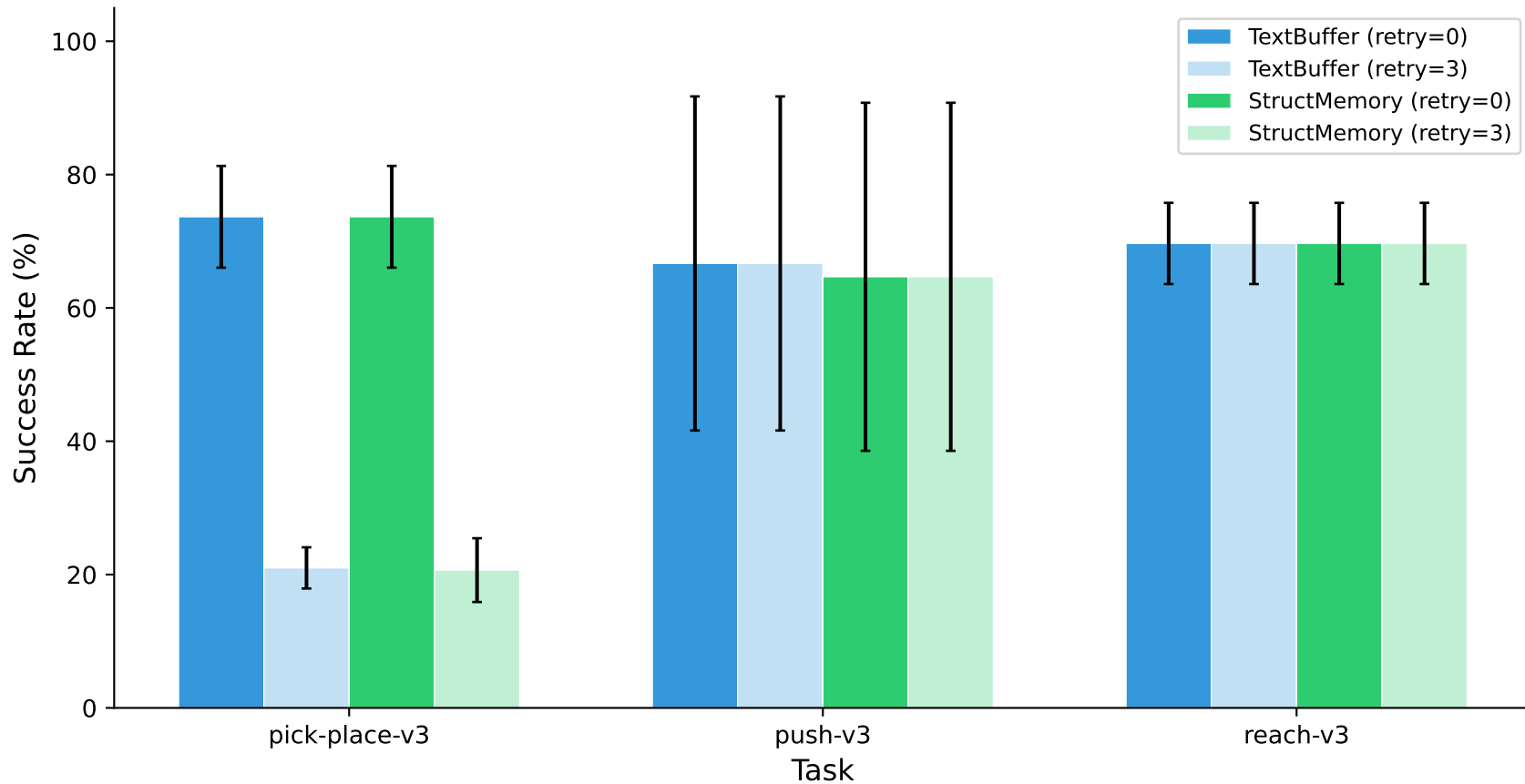
Fig 2: Retry=0 vs Retry=3 Comparison
