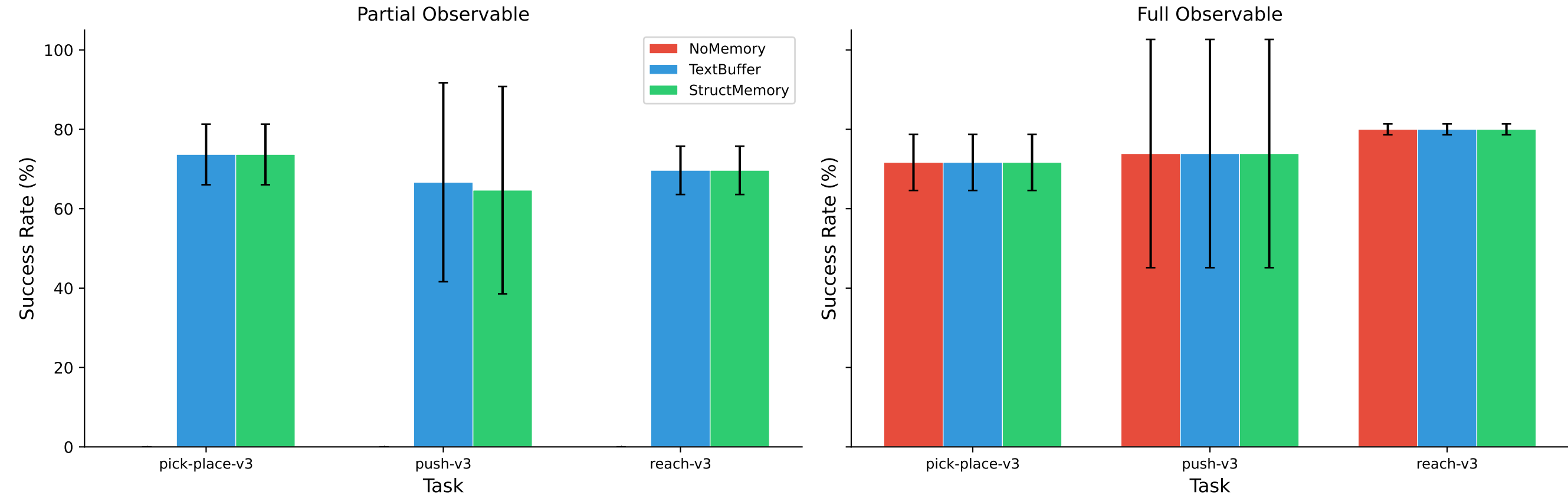
Fig 3: Partial Observable vs Full Observable
