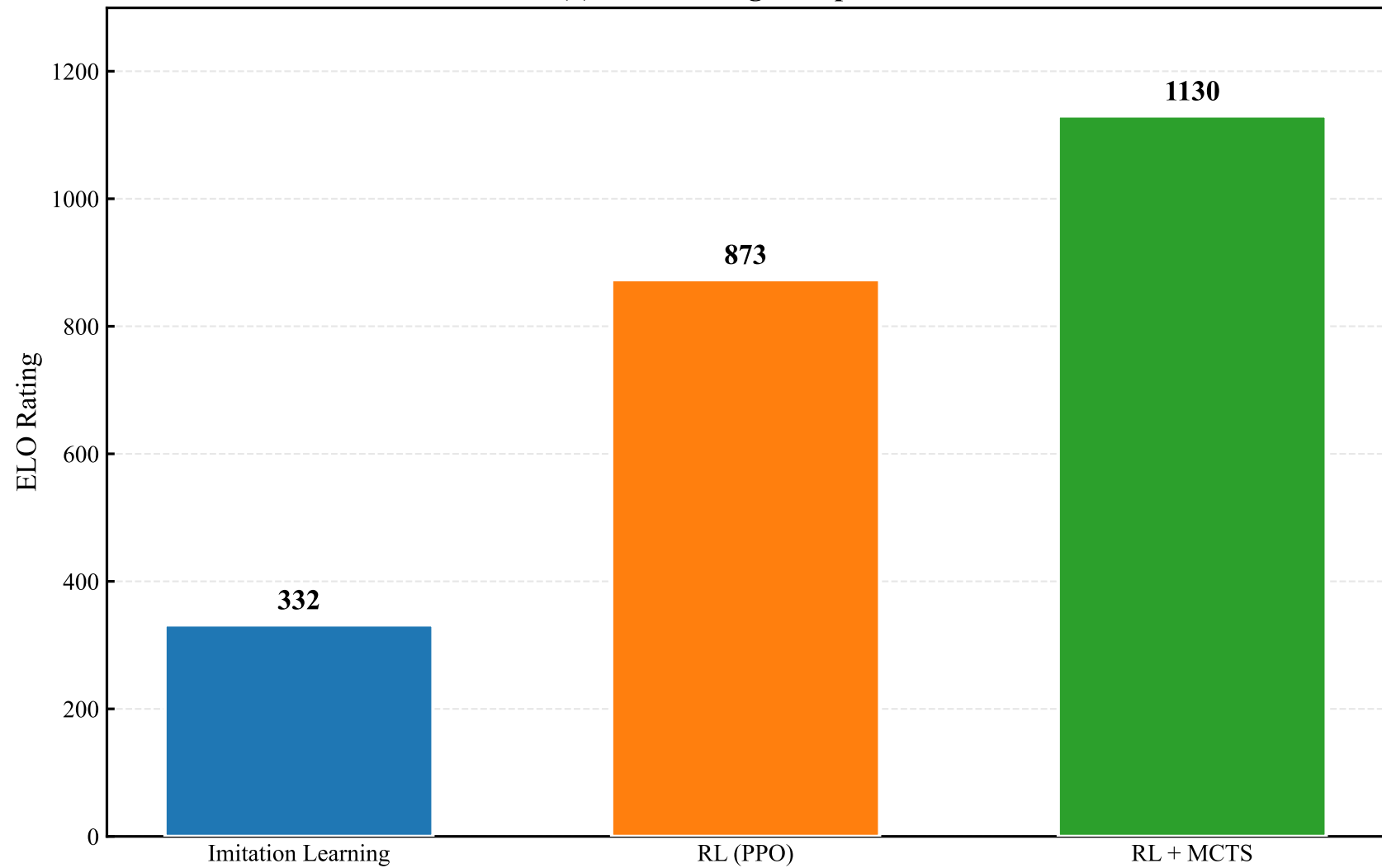
(a) ELO Rating Comparison
