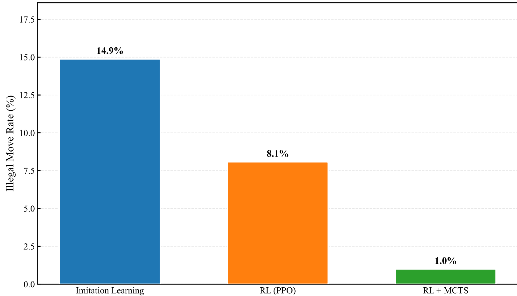
(b) Illegal Move Rate Comparison
