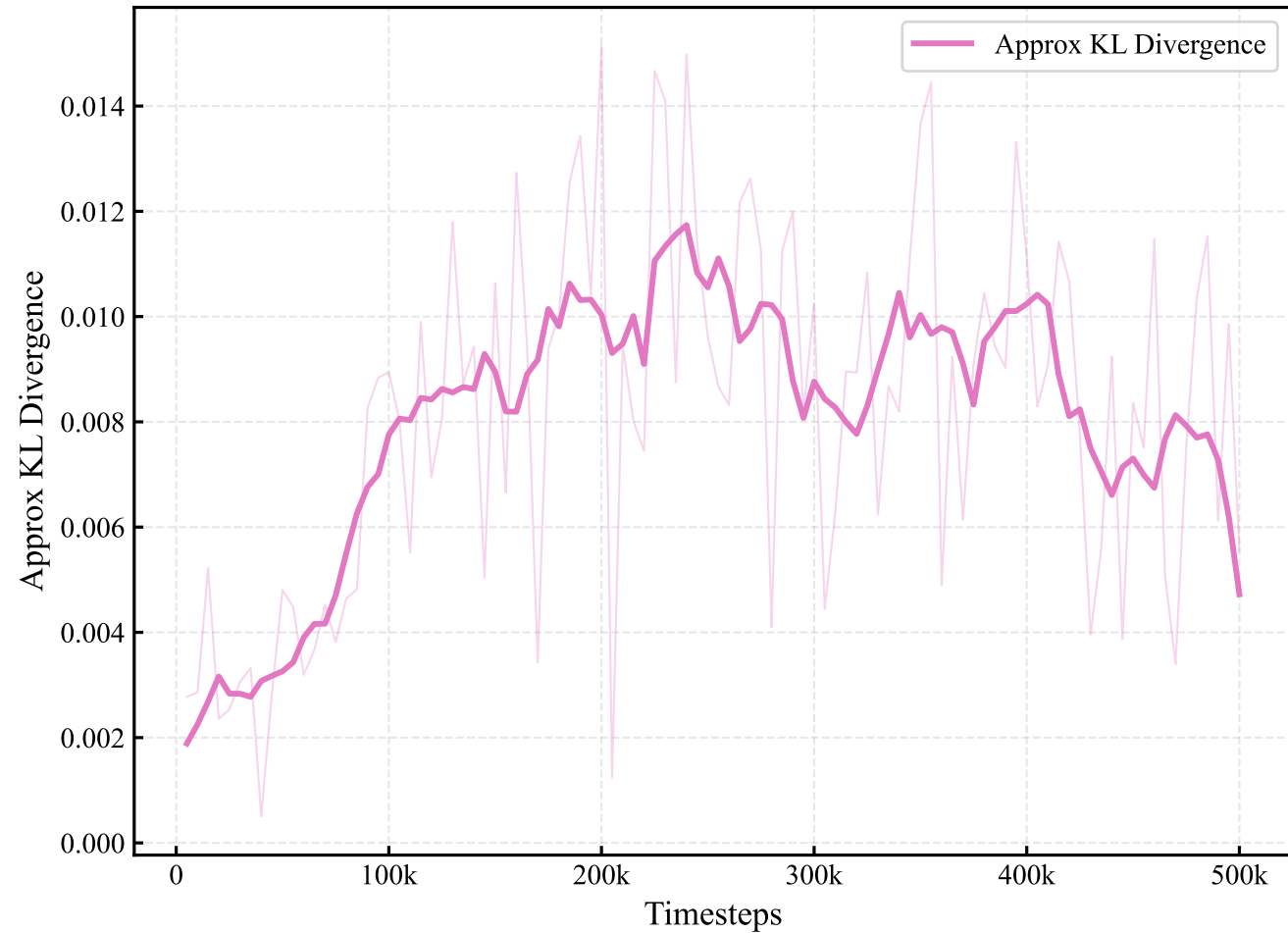
(a) Policy KL Divergence
