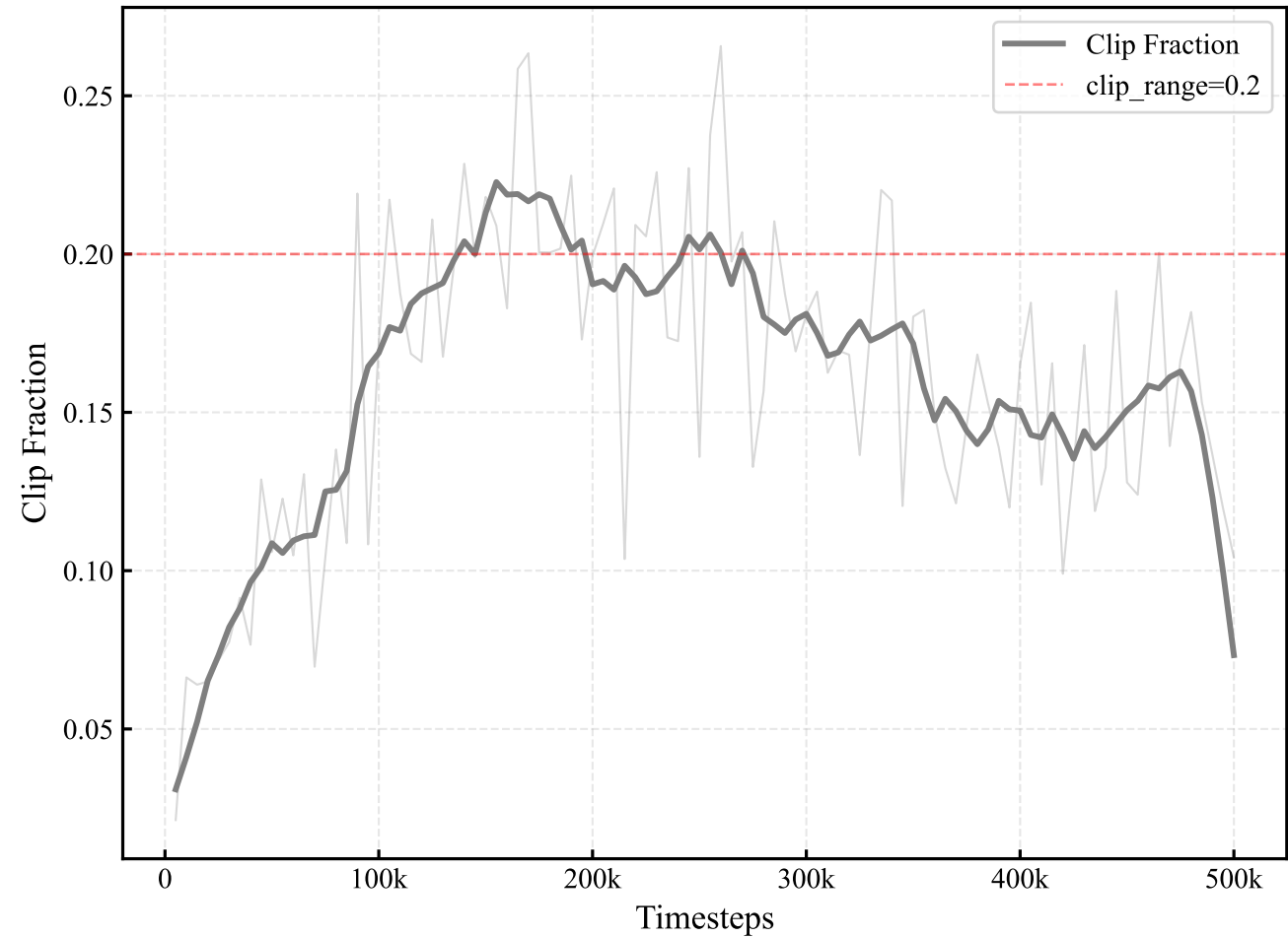
(b) Clipping Fraction
