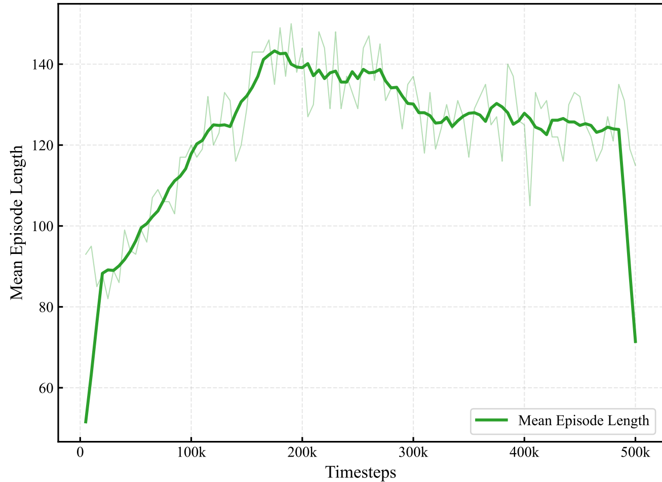
(b) Episode Length Curve
