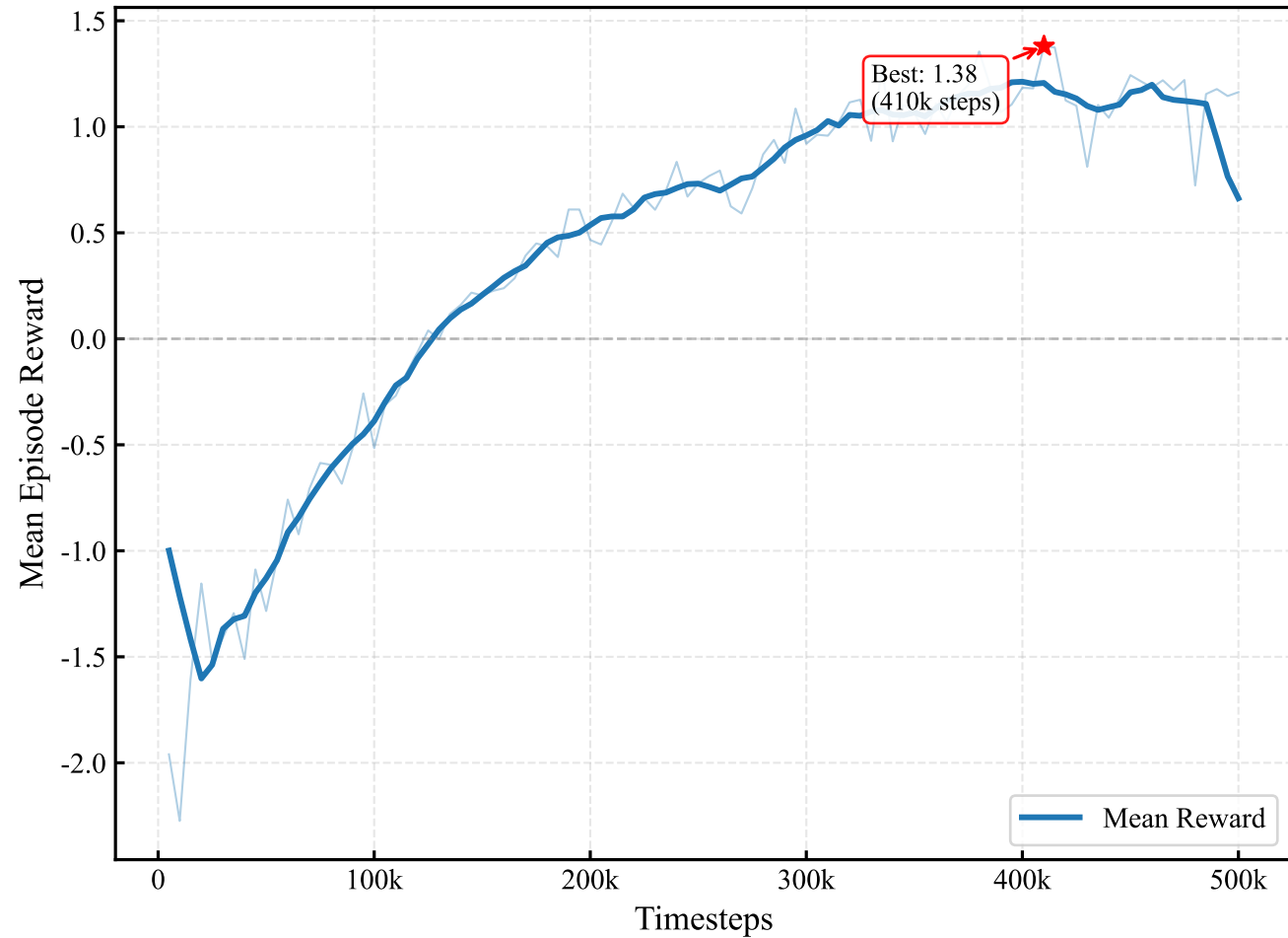
(a) Training Reward Curve
