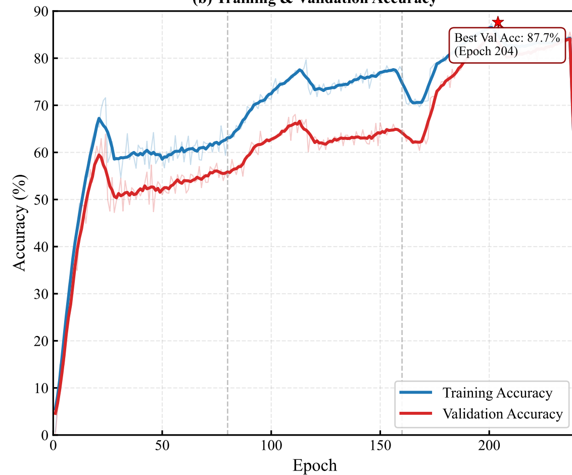
(b) Training & Validation Accuracy
