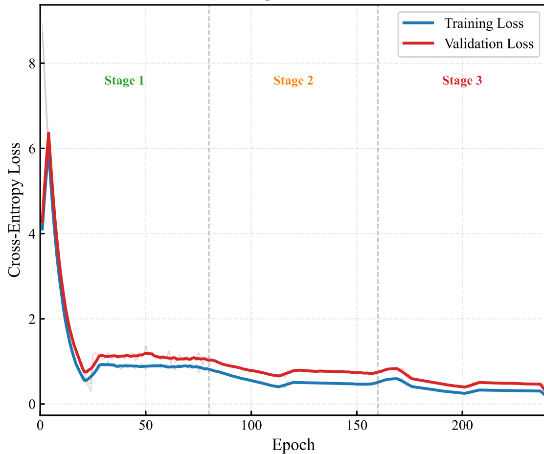
(a) Training & Validation Loss
