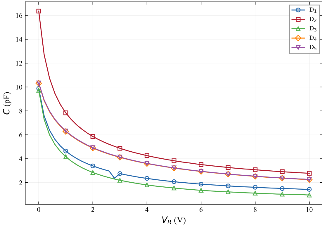
C--V Characteristics of All Diodes
