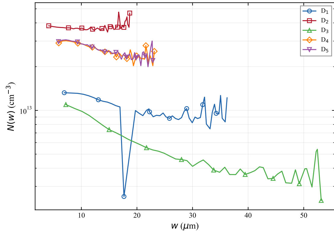
Impurity Concentration Profiles N(w)
