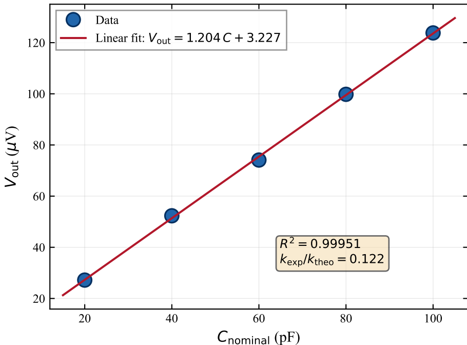
Lock-in Amplifier Calibration: V_{\text{out}} vs. C_{\text{nominal}}
