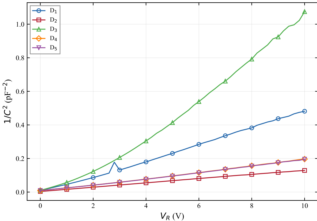
1/C^2 -- V_R Characteristics of All Diodes
