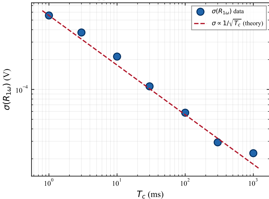
Noise Suppression vs. Lock-in Time Constant
