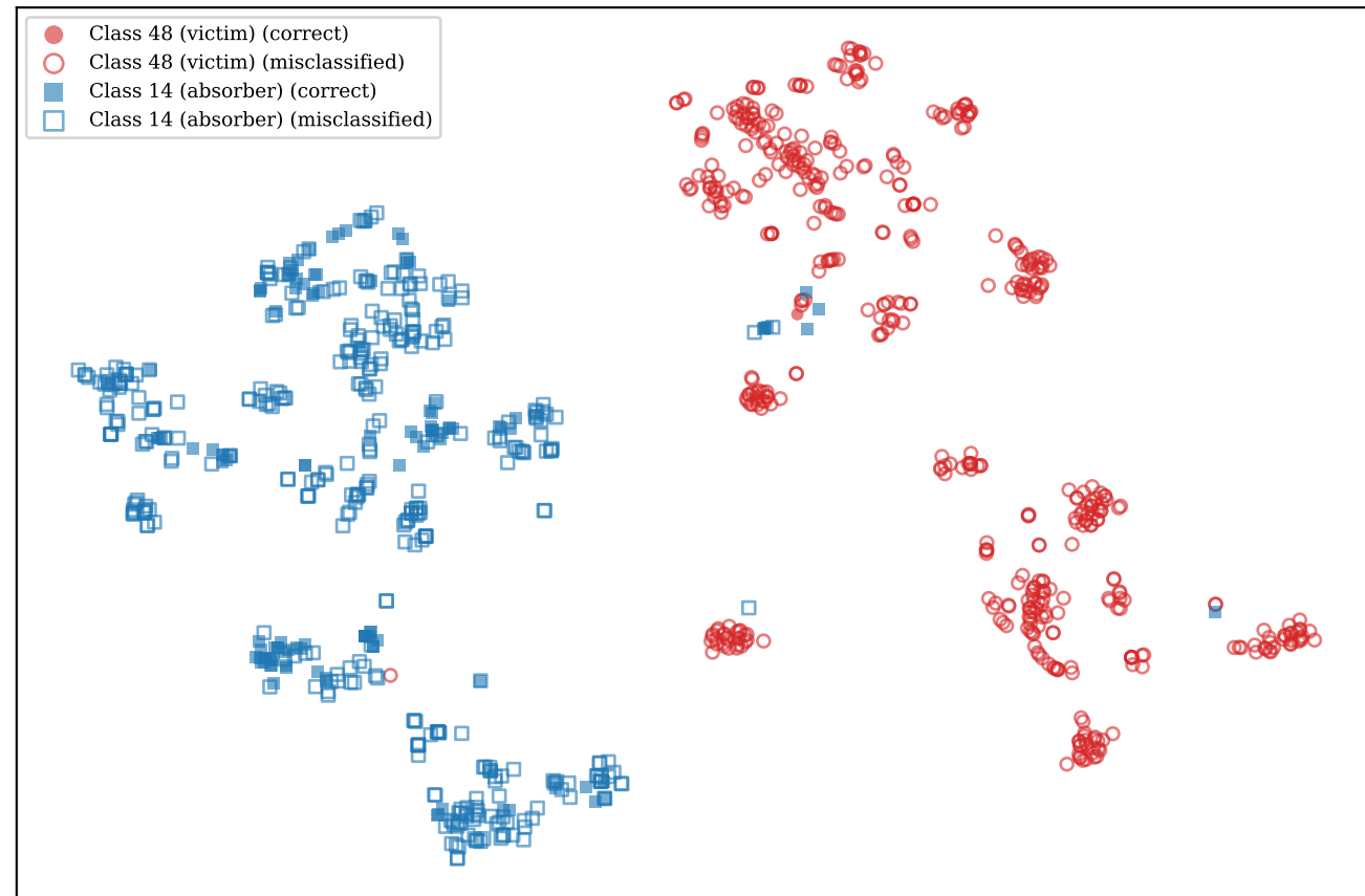
M-2022-12 (t-SNE) Victim 48 recall: 0.00
