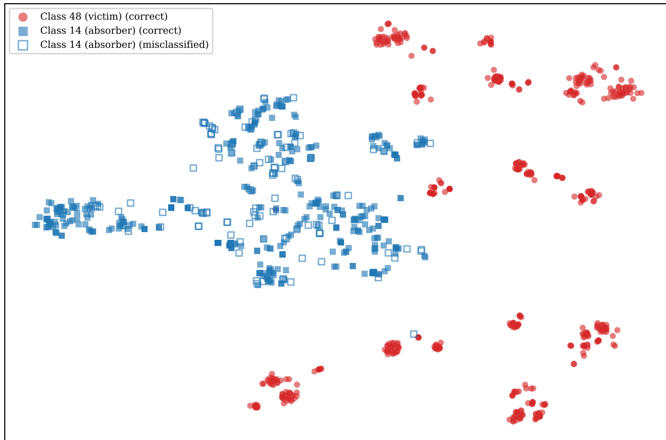
M-2022-3 (t-SNE) Victim 48 recall: 1.00
