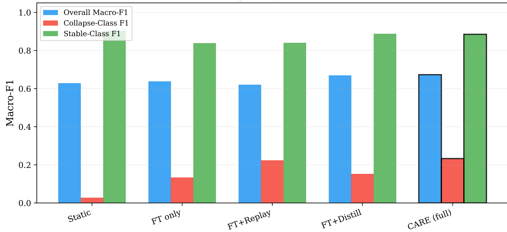
Ablation Study: Component Contribution
