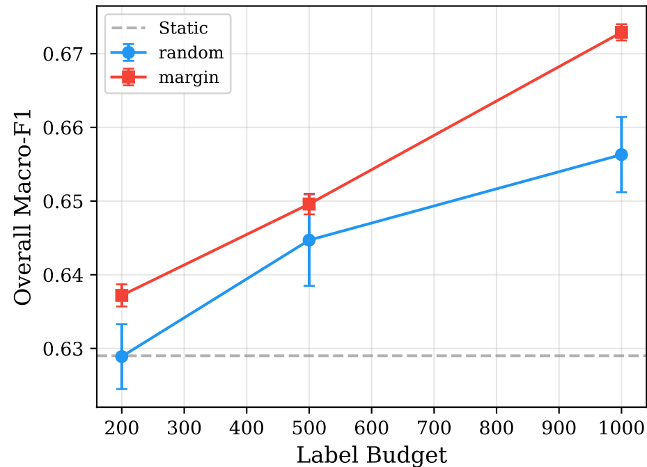
Label Efficiency: Macro-F1
