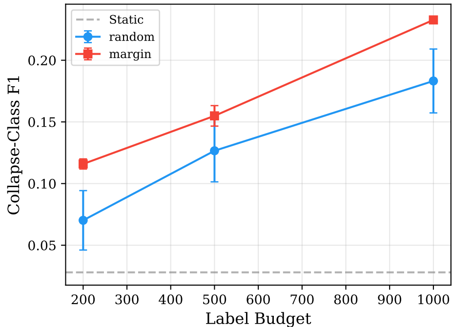
Label Efficiency: Collapse Recovery
