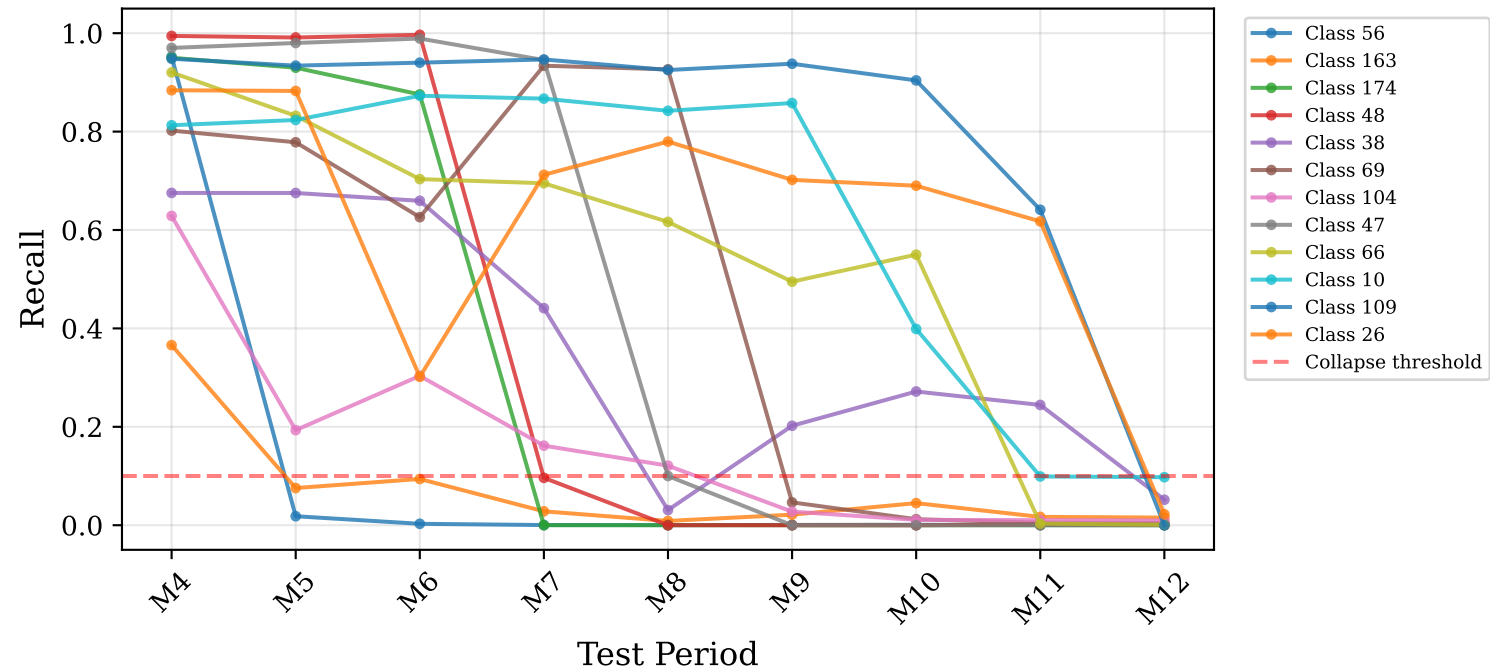
Recall Trajectories of Collapse Classes
