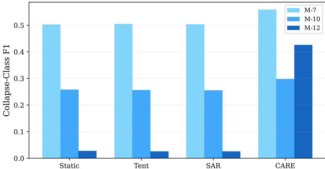
Collapse-Class F1 Across Time Points
