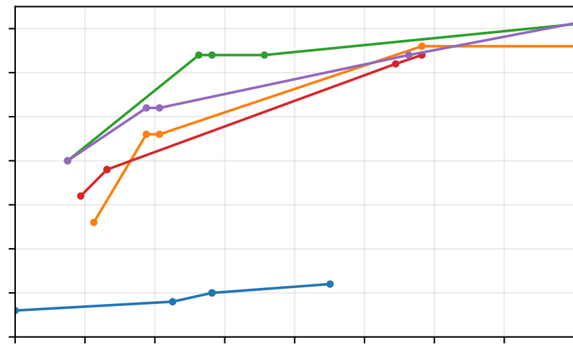
CWE399
