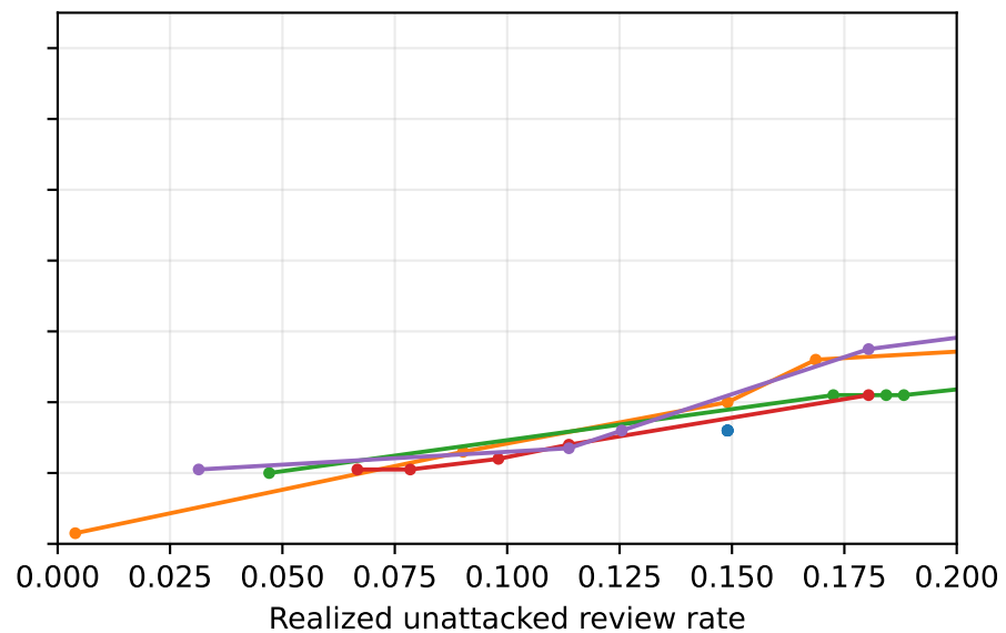
CWE399
