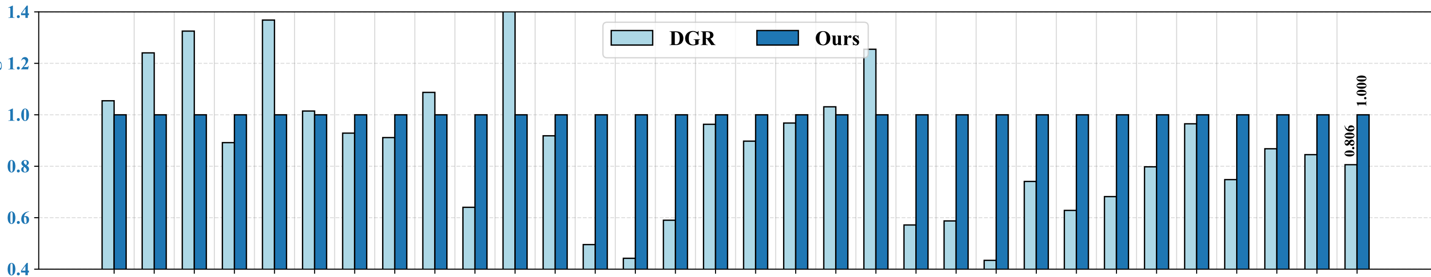
Normalized Pattern Routing Runtime
