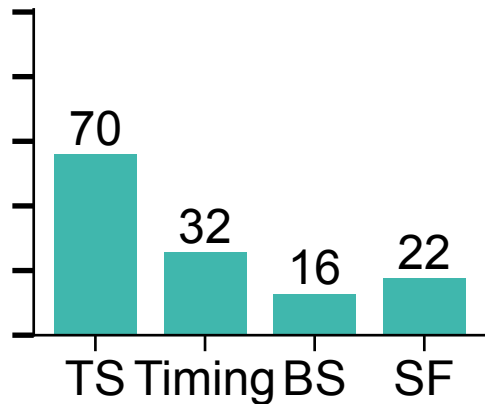
(c) Semantics
