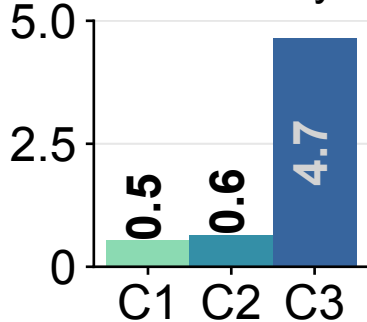
BPF verify
