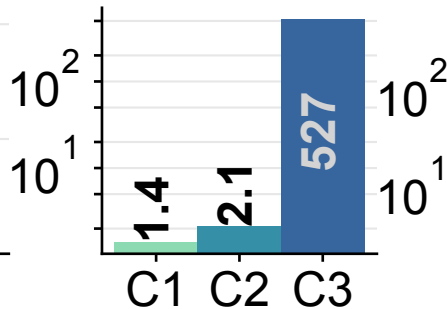
Kprobe Register
