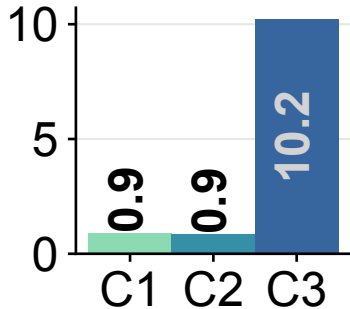
JMP Optimization
