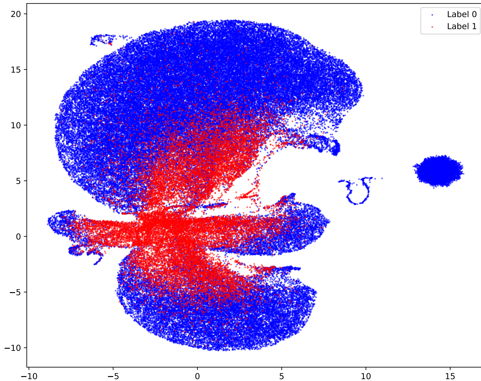
UMAP Visualization (True Labels)
