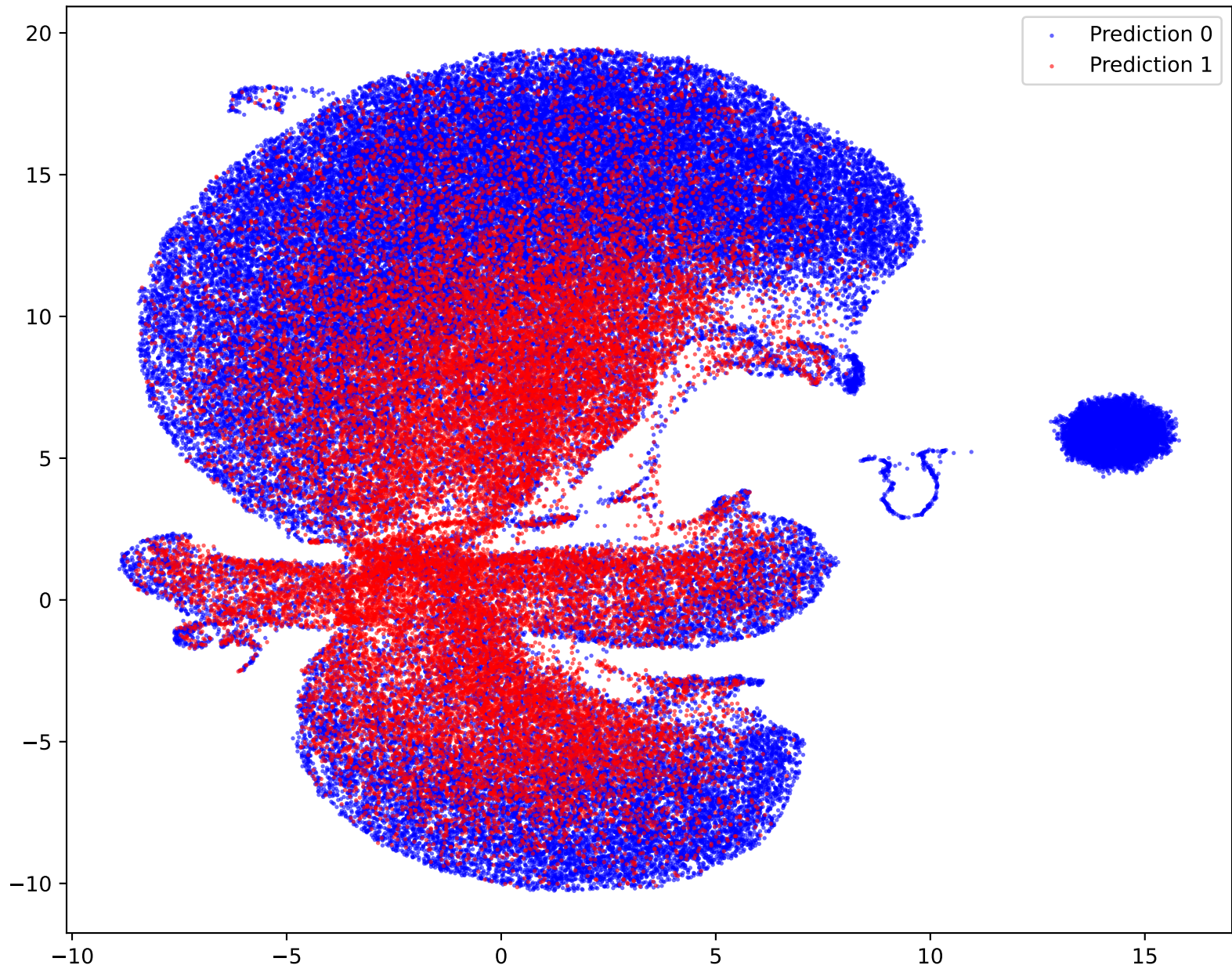
UMAP Visualization (Predictions)
