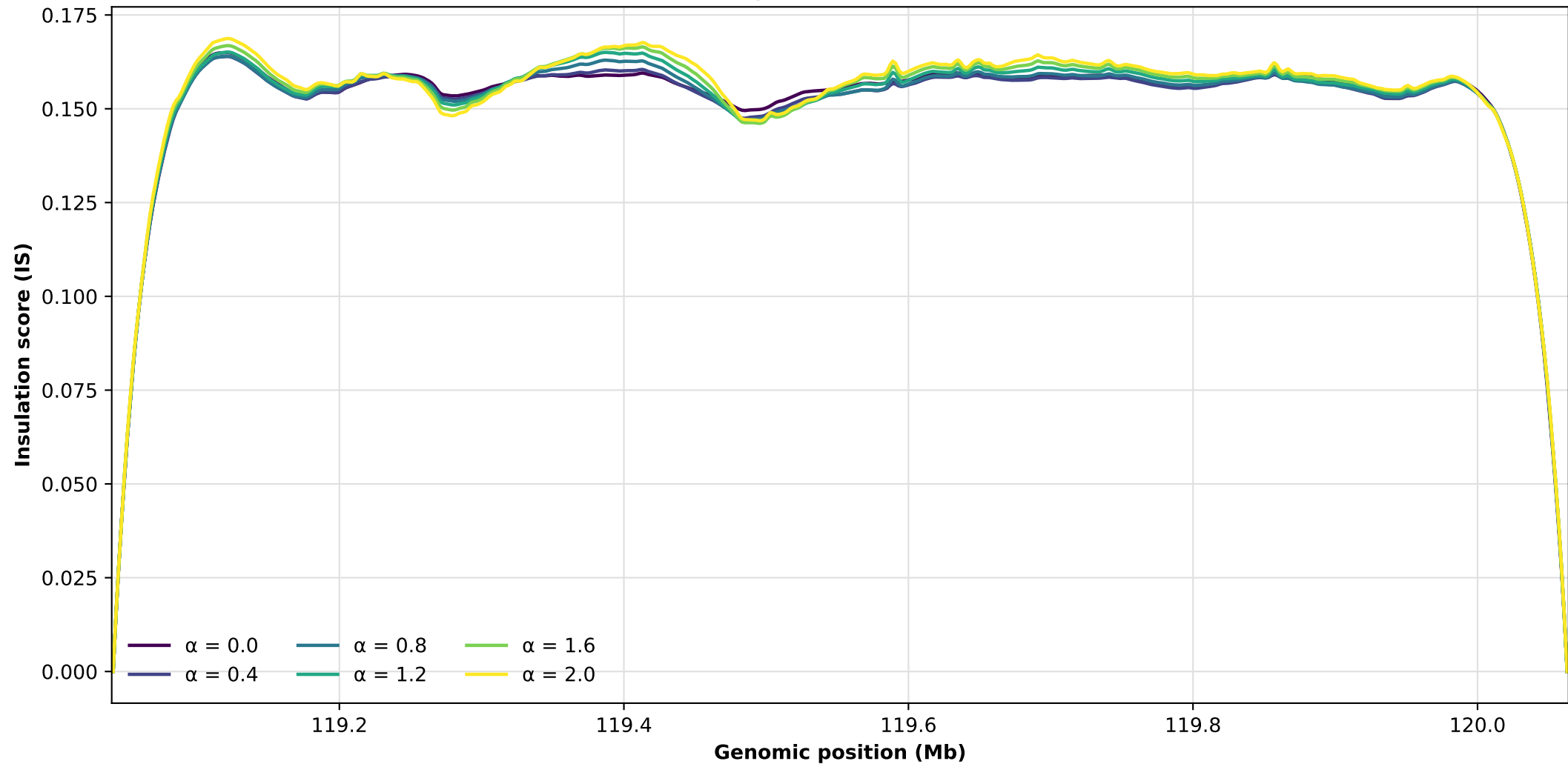
IS profiles across alpha: chr7_119040000_120064000 DNase scaling, 50-bin window (100 kb)
