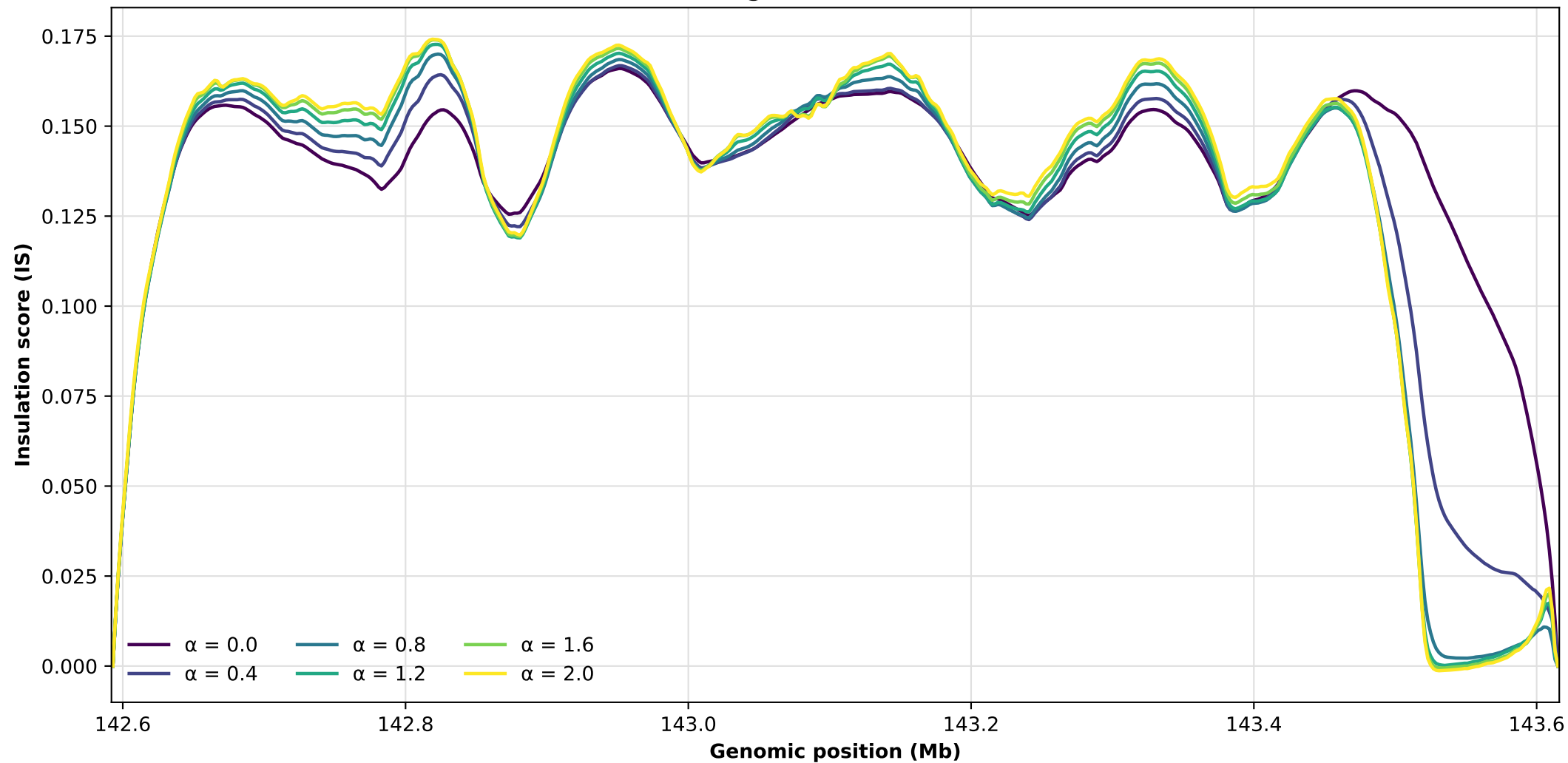
IS profiles across alpha: chr7_142592000_143616000 DNase scaling, 50-bin window (100 kb)
