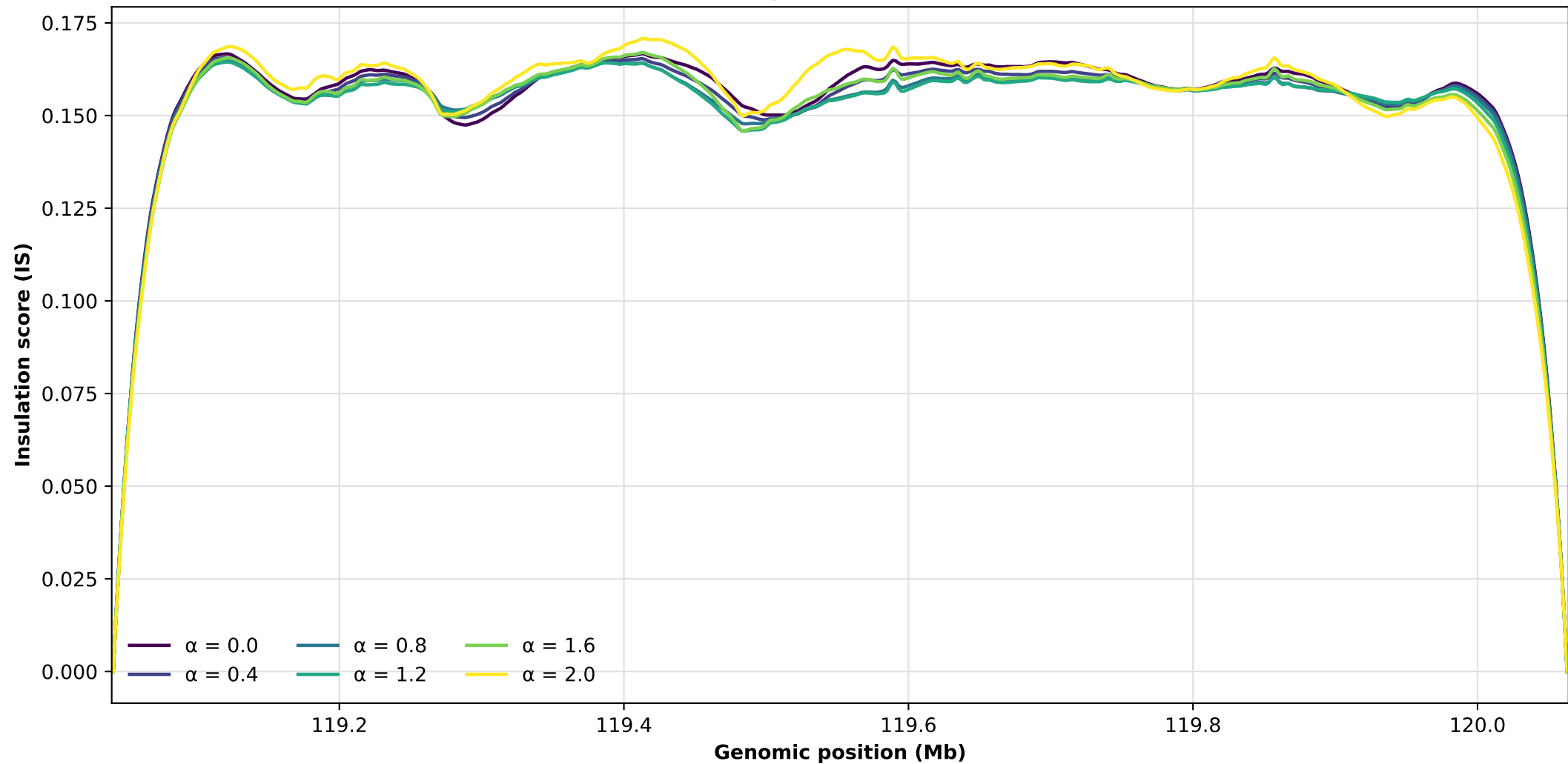
IS profiles across alpha: chr7_119040000_120064000 H3K27ac scaling, 50-bin window (100 kb)
