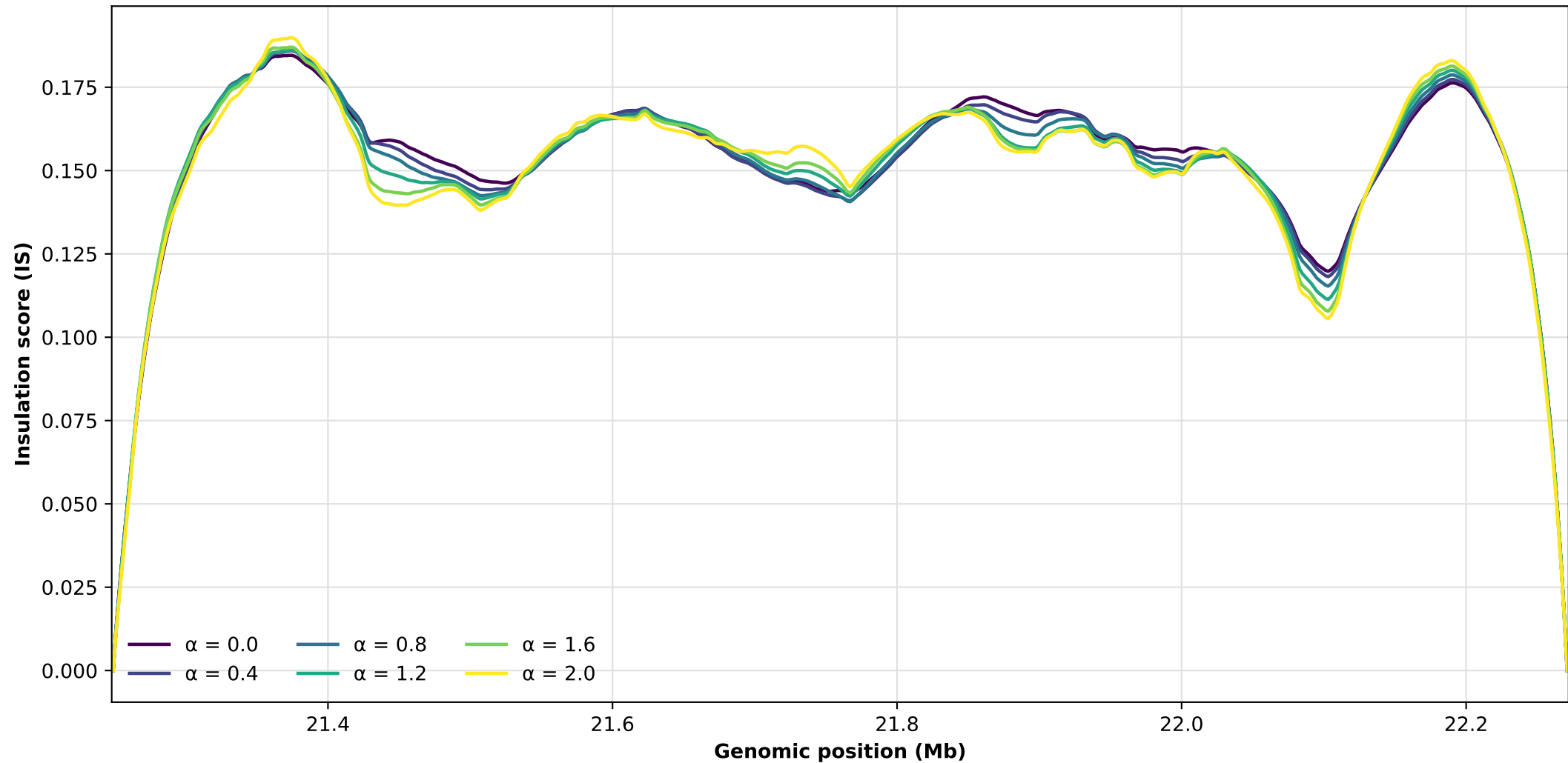
IS profiles across alpha: chr7_21248000_22272000 H3K27ac scaling, 50-bin window (100 kb)
