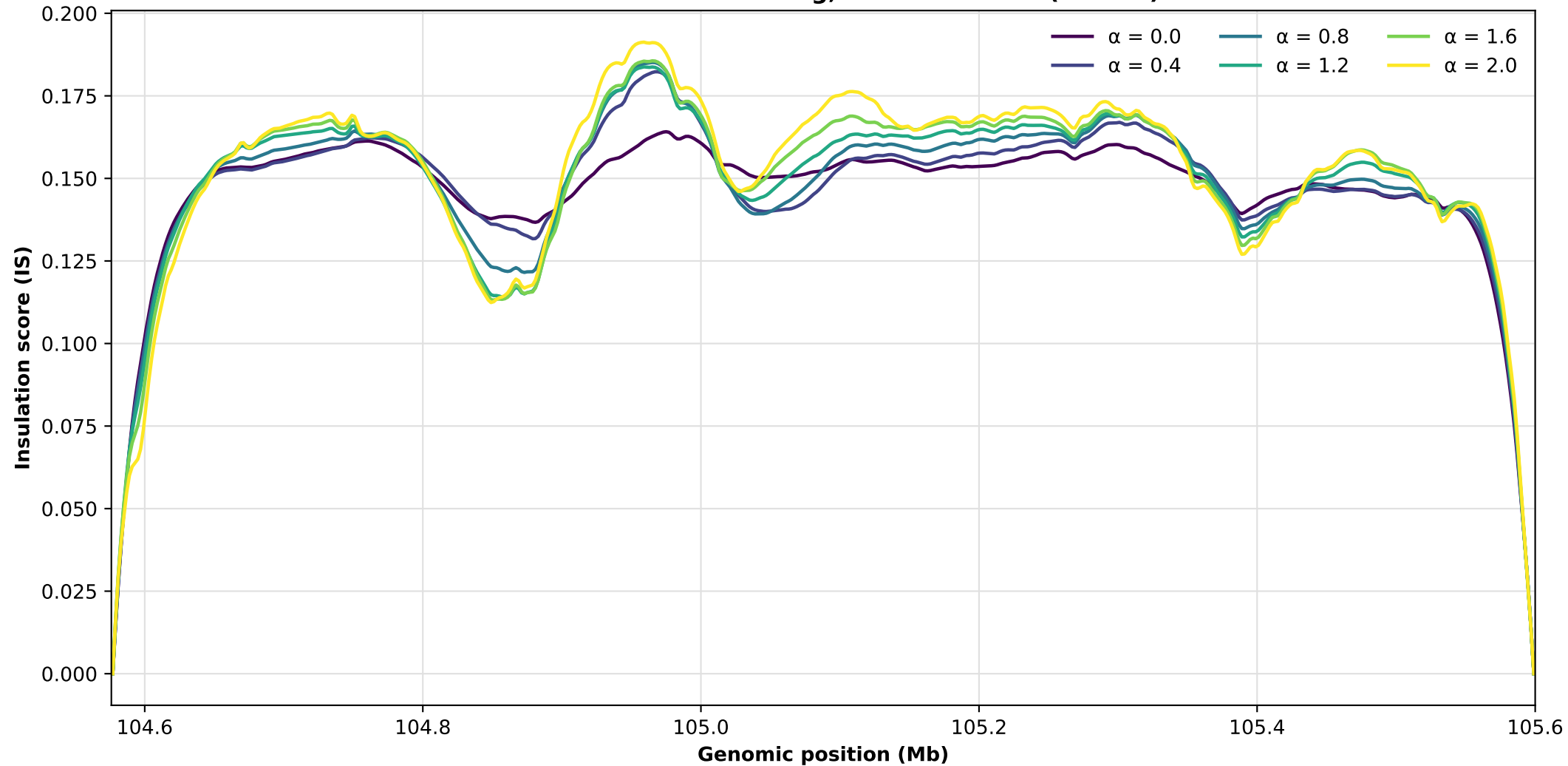
IS profiles across alpha: chr7_104576000_105600000 DNase + H3K27ac scaling, 50-bin window (100 kb)
