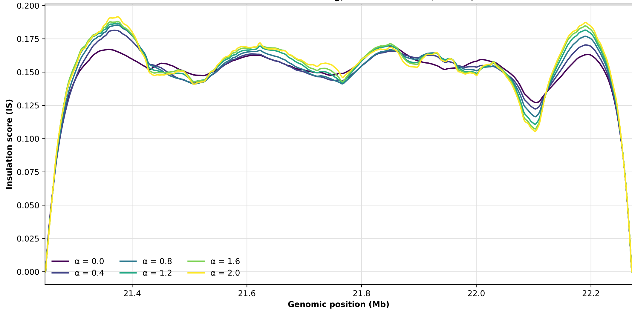
IS profiles across alpha: chr7_21248000_22272000 DNase + H3K27ac scaling, 50-bin window (100 kb)
